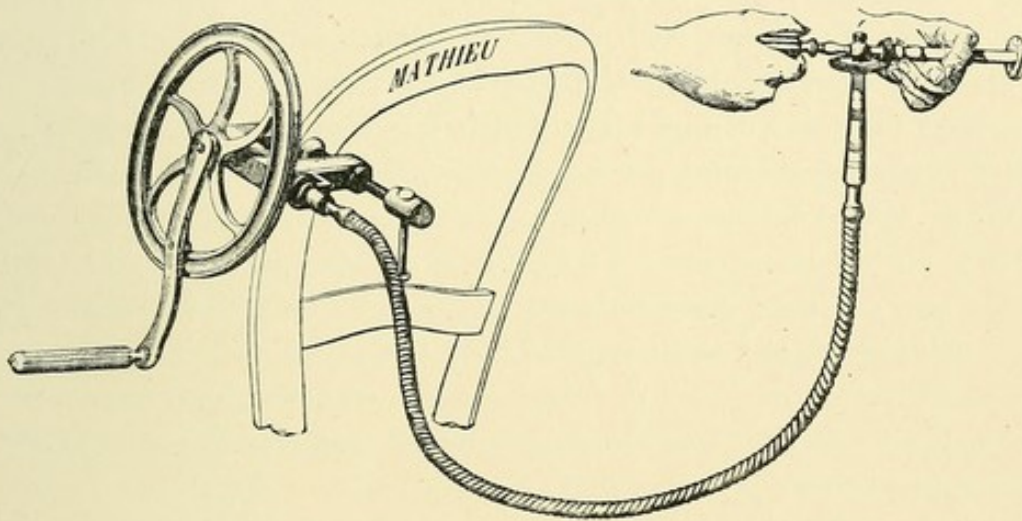
FIG. 209. — Scie rotative.
