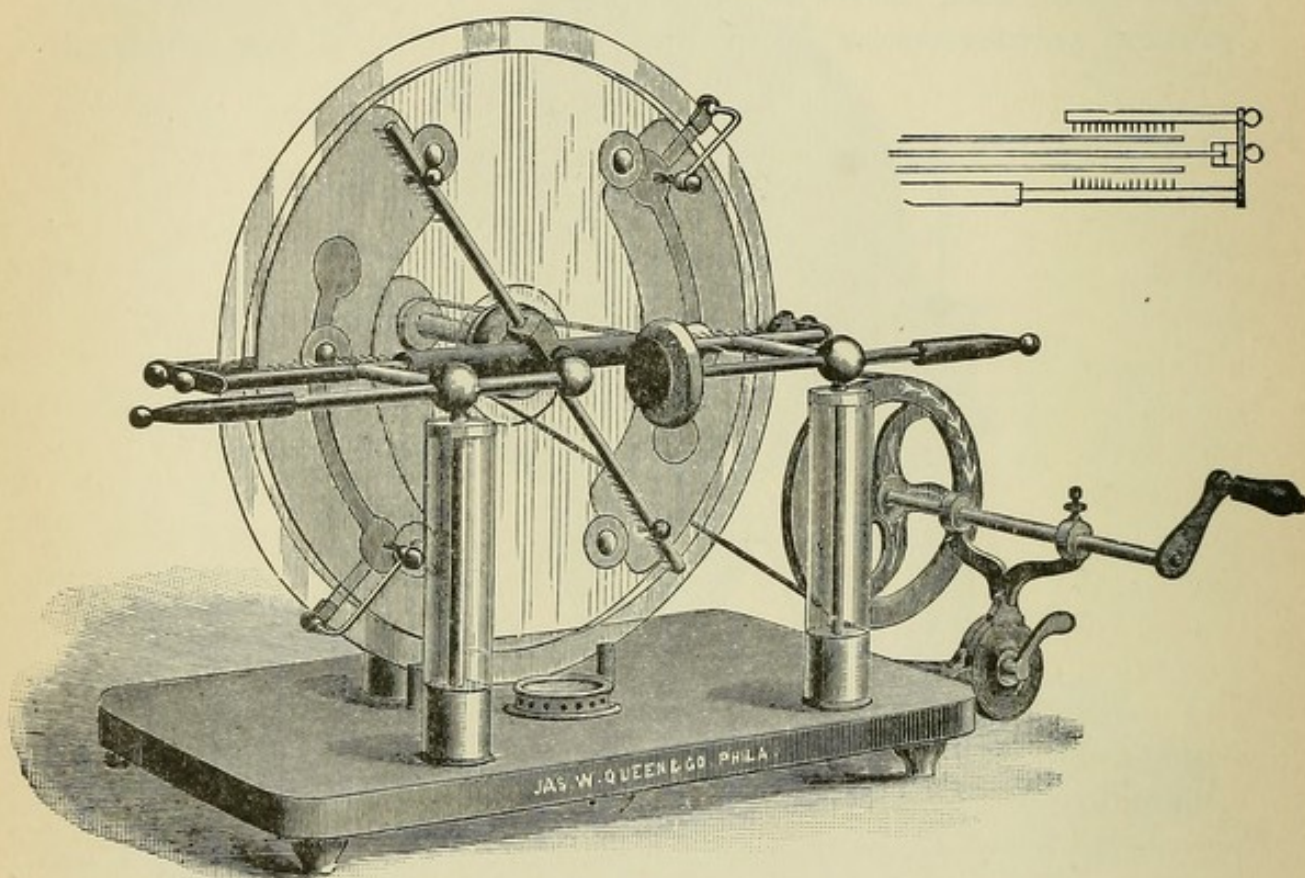
FIG. 11.—Toepler-Holtz influence machine.
