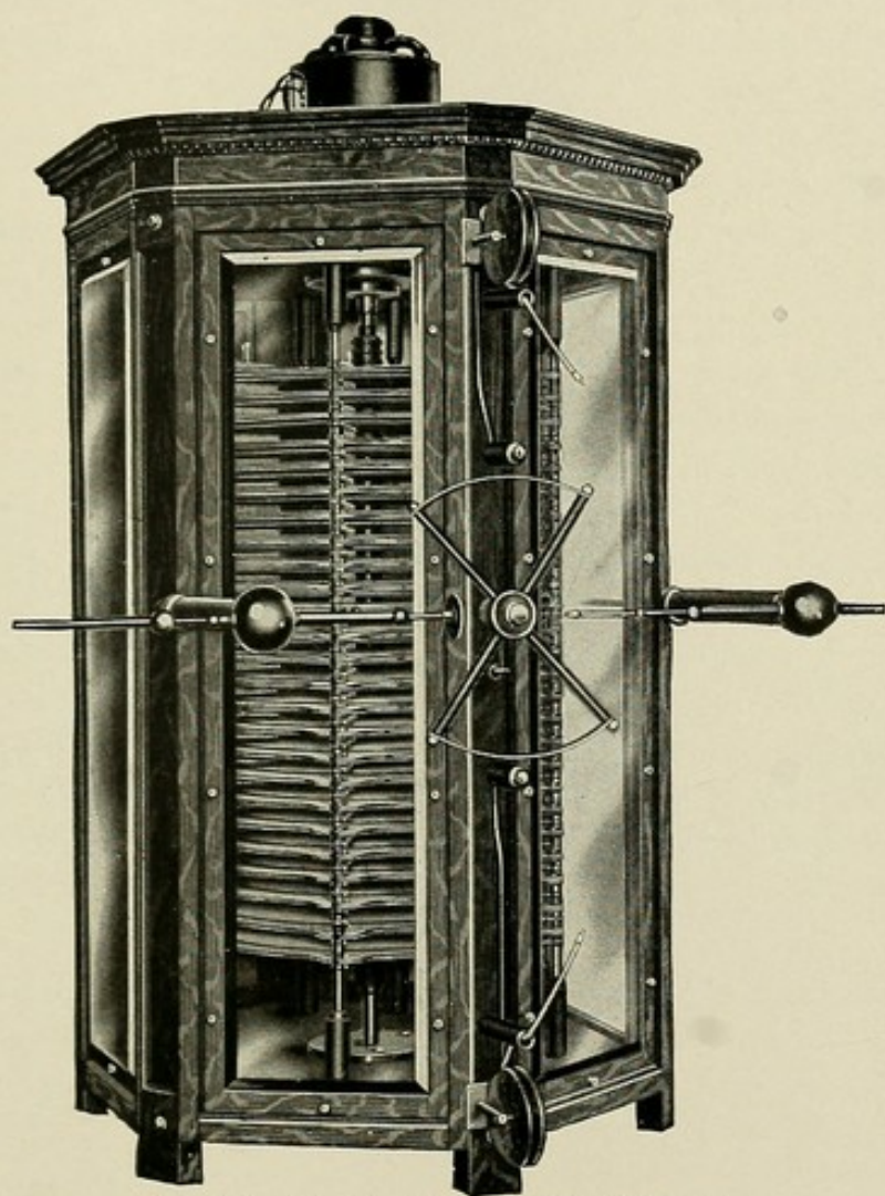
FIG. 81G.—100-plate static machine of Wagner.
