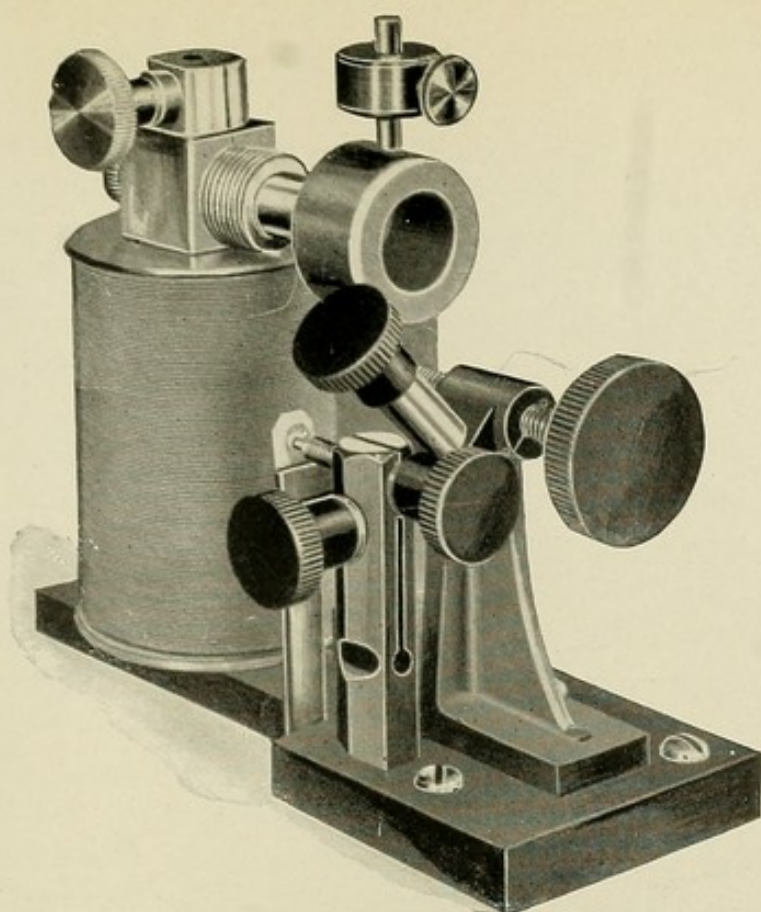
FIG. 69.—Self-starting interrupter.
