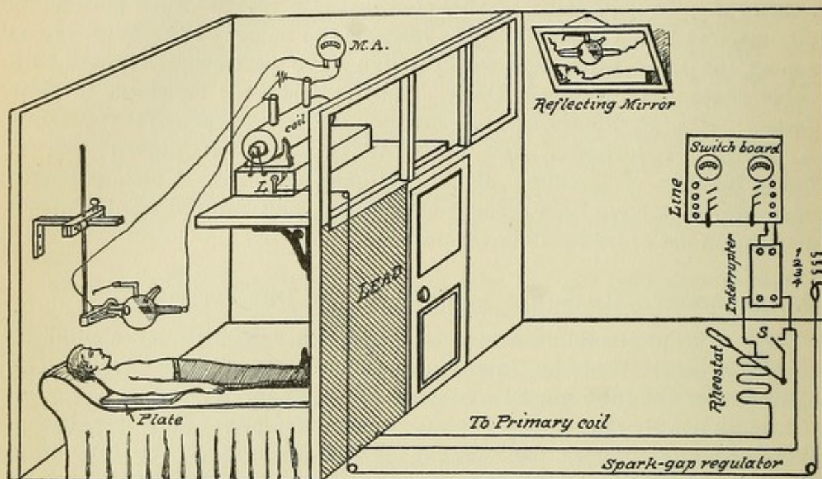
FIG. 210.—Author's scheme for the operator's protection.
