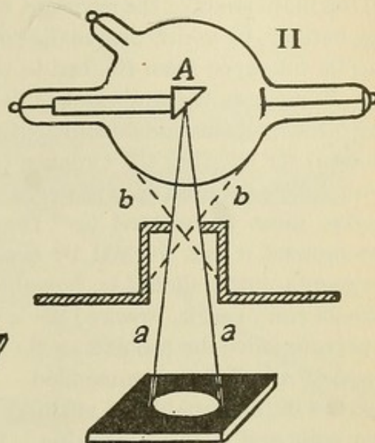
FIG. 99.—Tubular or compression diaphragm. (Donath.)
