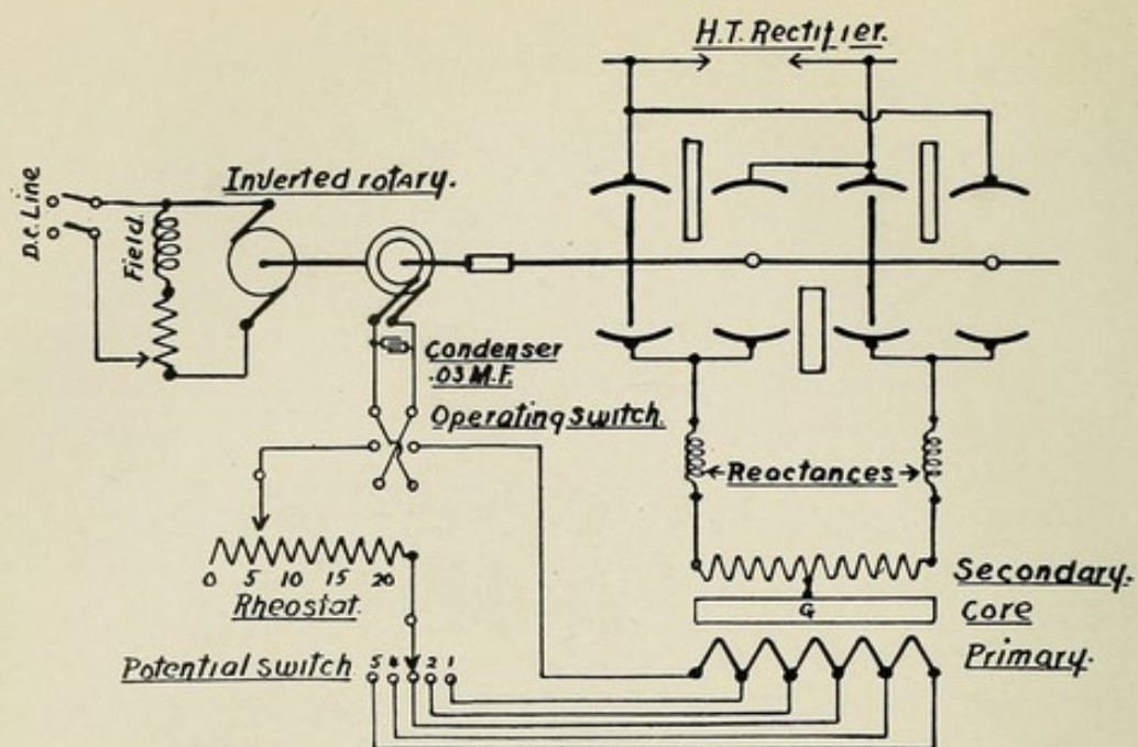
FIG. 81B.—Diagrammatic view of the Snook Röntgen Apparatus.
