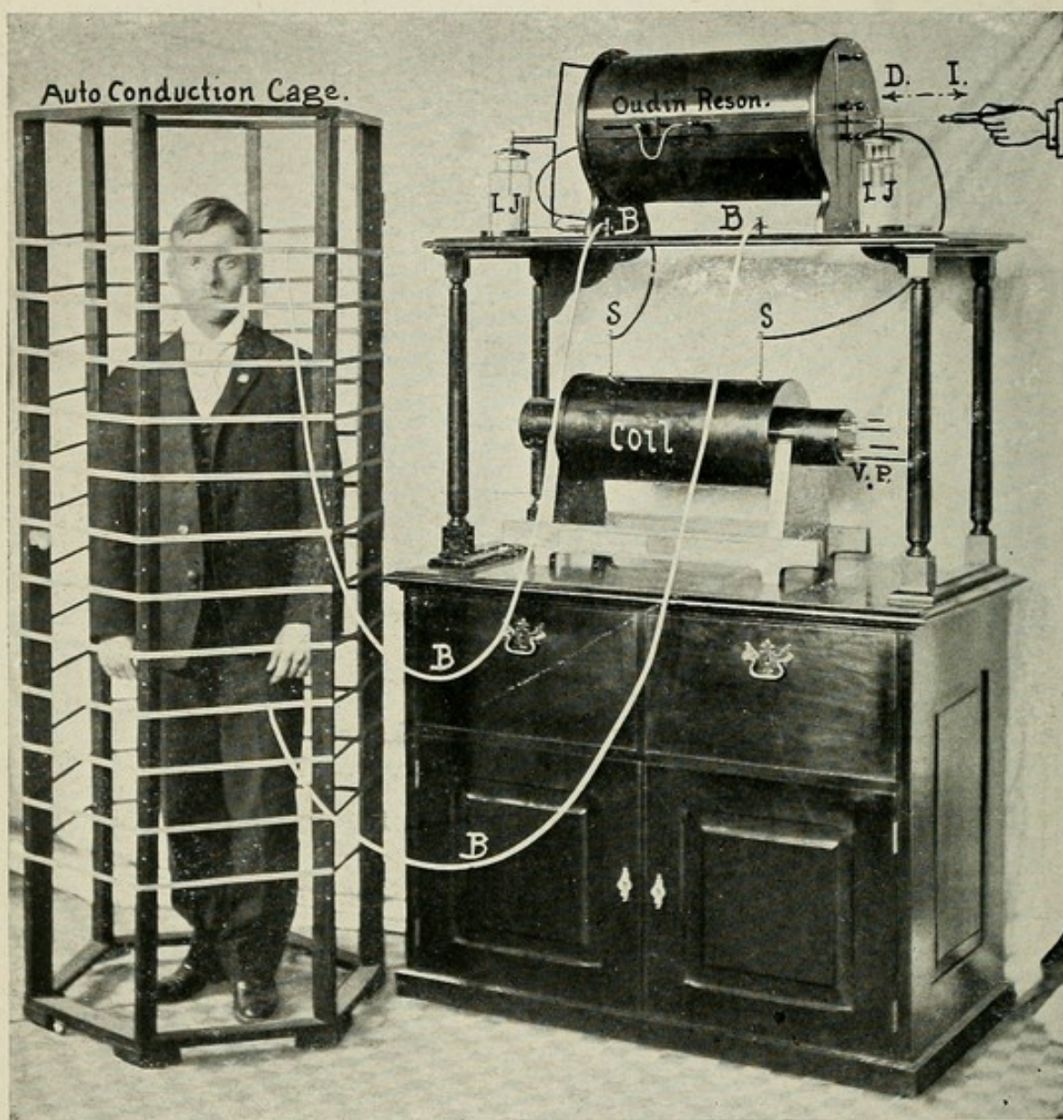
FIG. 66A.—Treatment by auto-induction. S S , secondary terminals of induction coil; B B , cords to the auto-conduction cage from the Oudin resonator; L J , Leyden jar; D \longleftrightarrow I , spark-gap; when sliding in the direction " D ," the current suffers a loss in intensity, and vice versa.
