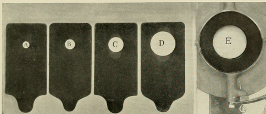
FIG. 210A.—DIAMETER OF DIAPHRAGMS.—Because of the immobilization of the part and its power of cutting the secondary rays, I have within the past year resorted in certain special cases to the compression diaphragm, although heretofore I was not one of its advocates. The following are the different distances for X-ray radiographic work, and also for therapy, taking the different sizes of diaphragms as here photographed in alphabetical order:
