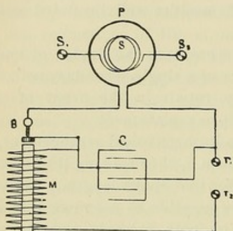
FIG. 77.—The Tesla oscillator.
