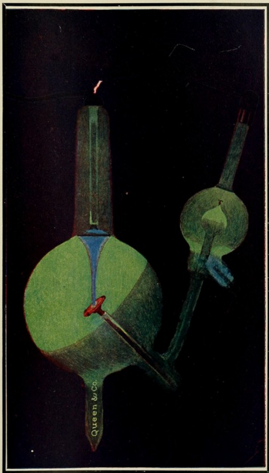
SELF-REGULATING X-RAY TUBE. LOW VACUUM. (FIG. 96.)
