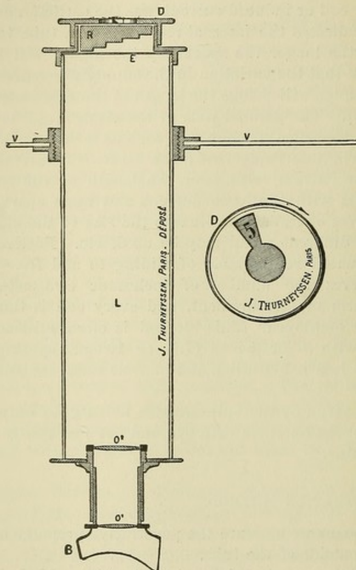
FIG. 216.—Benoist's radiochromometer.
