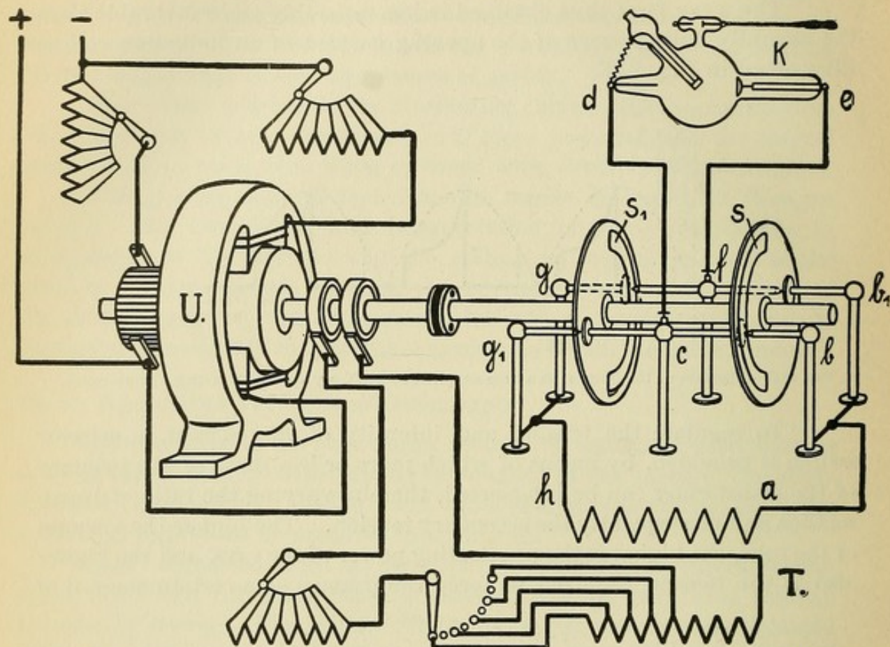
FIG. 81F.—Diagrammatic view of X-ray apparatus without an interrupter, for converting the direct into an alternating current.
