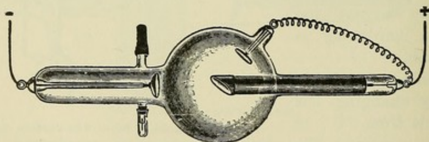
FIG. 92.—Osmosis regulating tube of Gundelach.
