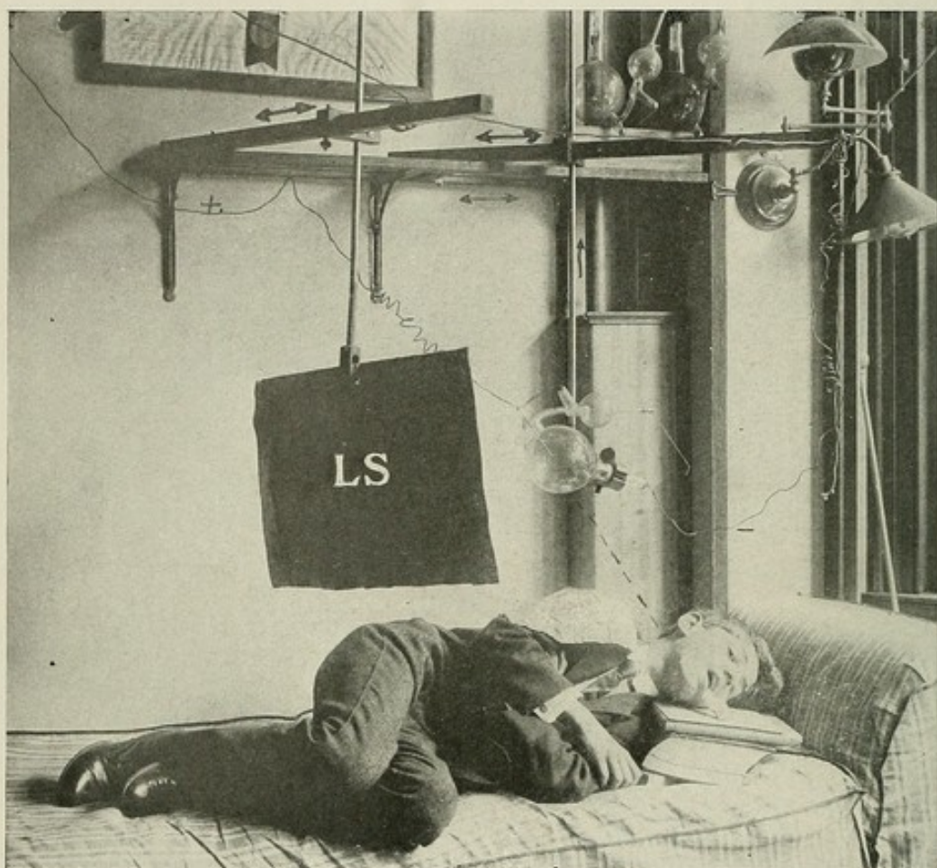
FIG. 200.—EXTRA-ORAL METHOD IN DENTAL SKIAGRAPHY.—LS, lead screen for the protection of the operator. The arrows indicate the variable positions to which the author's tube-holder may be shifted. The illustration depicts the sensitive plate placed upon a book and the lad's left (suspected side) cheek resting on the plate, the dotted line shows the path of the rays.
