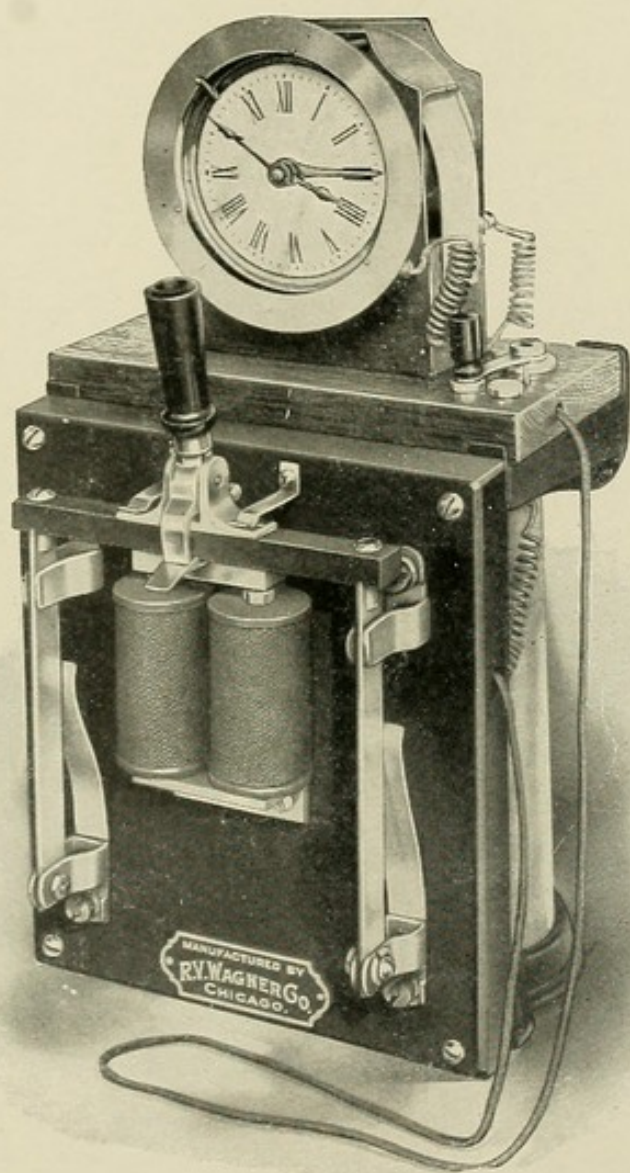
FIG. 103A.—Wagner's automatic switch.
