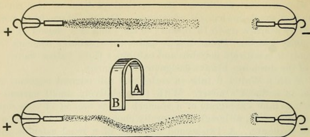
FIGS. 82, 83.—Discharge passing through low-vacuum tubes. (Bouchard.)
