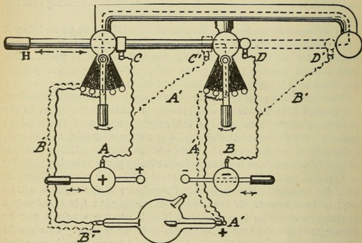
FIG. 16.—Pole changer of Betz.
