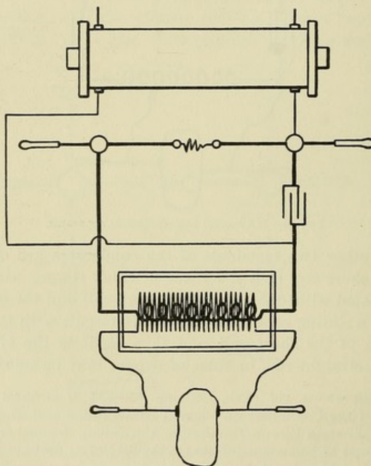
FIG. 60.—The Tesla transformer.
