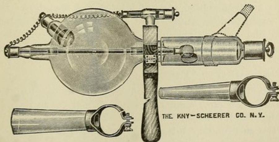
FIG. 213.—THE KNY-SCHEERER TUBE.—The anode is placed into the tubular extension, the latter being encased by a cylinder of lead-flux glass. A set of two specula of lead glass further serve to localize the X-rays.
