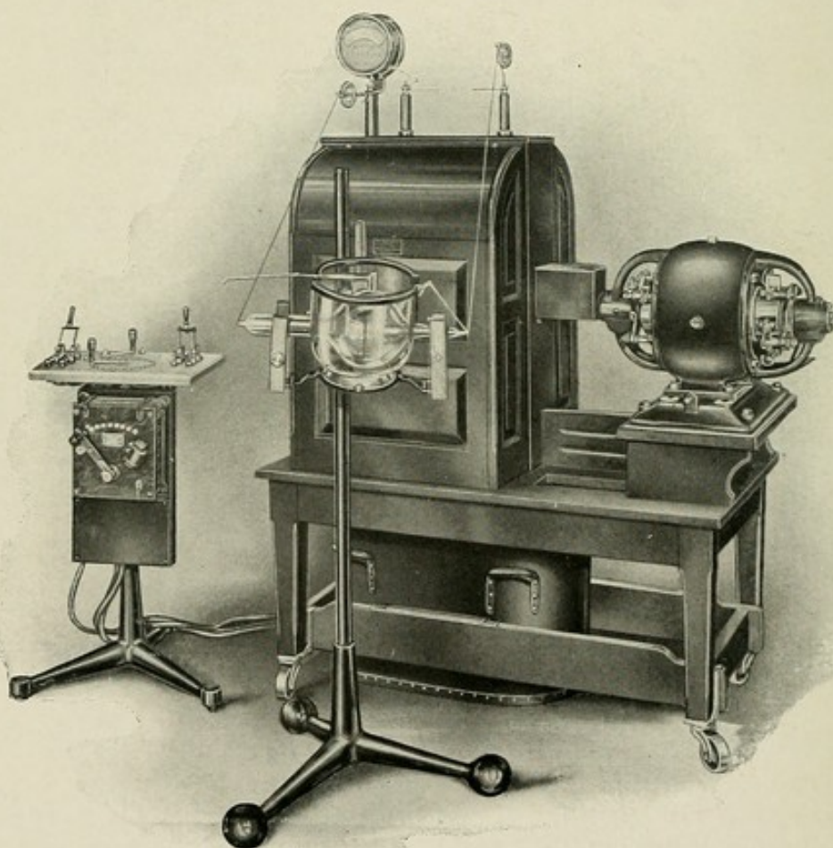
FIG. 81C.—The Snook Röntgen Transformer.
