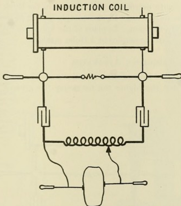
FIG. 59.—D'Arsonval high-frequency apparatus.
