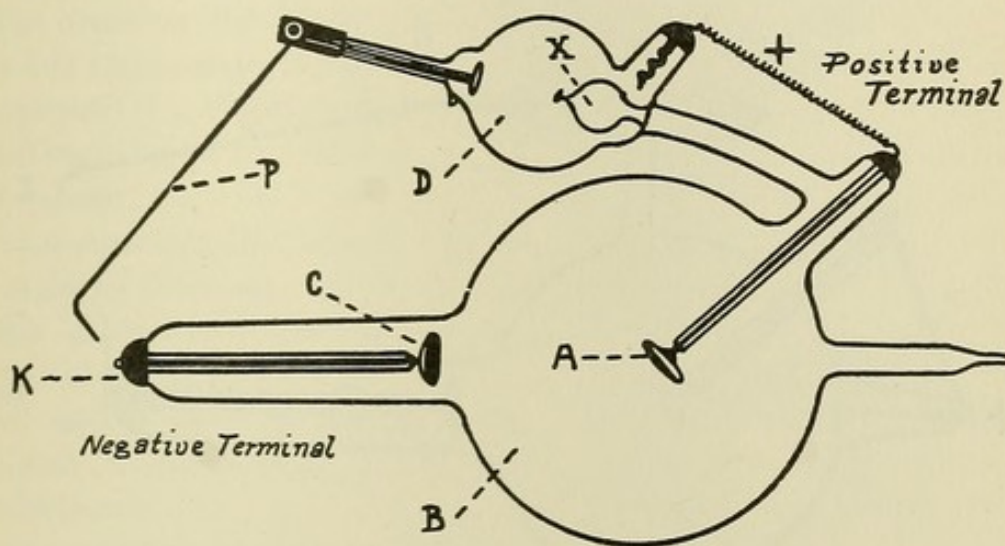
FIG. 89.—Queen's self-regulating tube.
