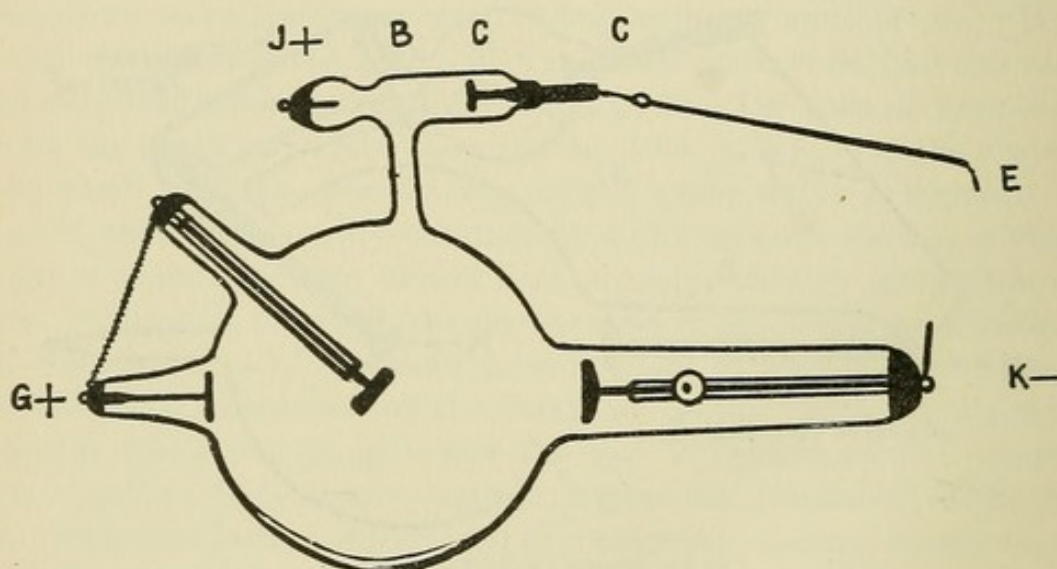
FIG. 90.—Müller's regulation tube. •
