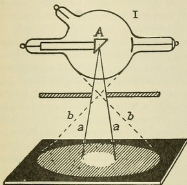
FIG. 98.—Ordinary diaphragm.
