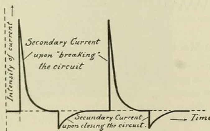
FIG. 81E.—Diagram of the current in a tube supplied by an induction coil.
