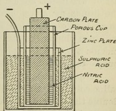
FIG. 24.—Bunsen cell (double fluid).
