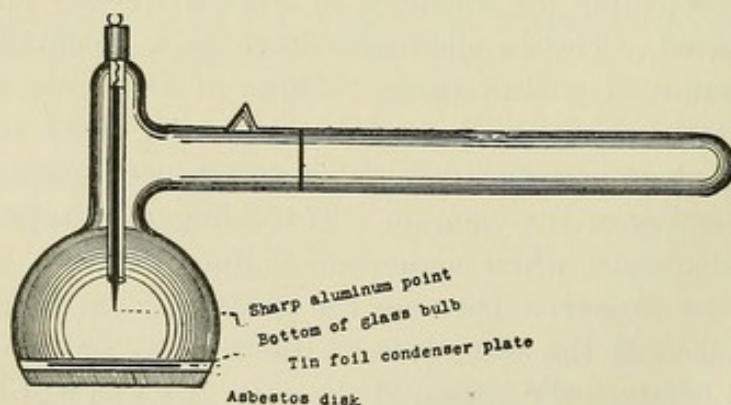
FIG. 65.—Morton's cataphoric electrode. (Waite & Bartlett Manufacturing Co.)
