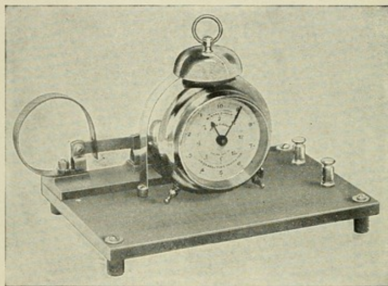
FIG. 103B.—TIME SWITCH.—This time switch may be used to stop automatically the coil, static machine, vibrator, or therapeutic lamp at the end of a treatment: especially valuable where two or more patients are treated at the same time. The switch proper is of the single pole knife variety. The contacts are substantial and there is no possibility of sticking. I found it very satisfactory in my practice.
