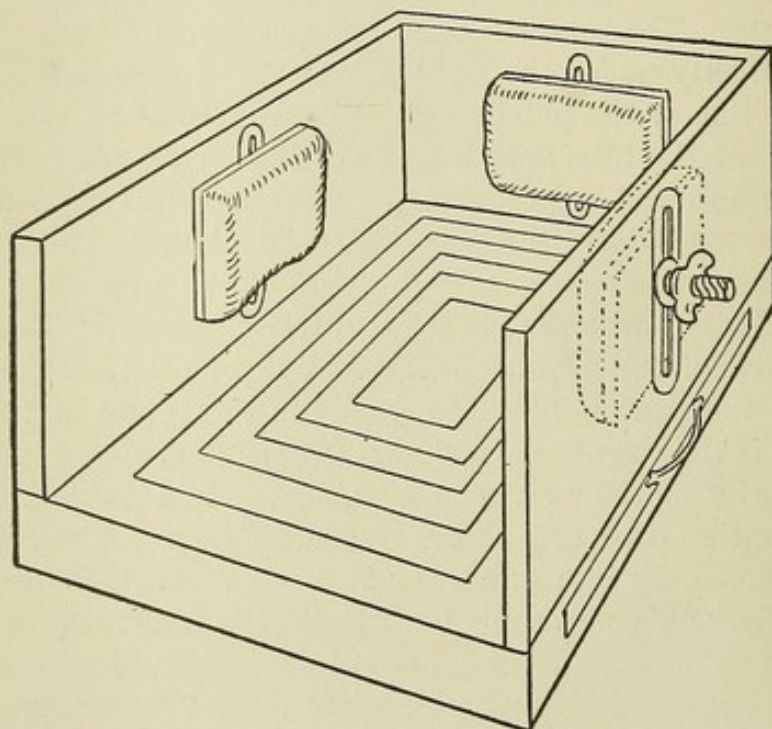
FIG. 197.—Author's head rest for stereoscopic work.
