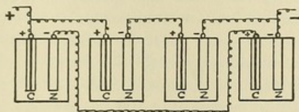
FIG. 4.—Connection of the cells in “groups.”
