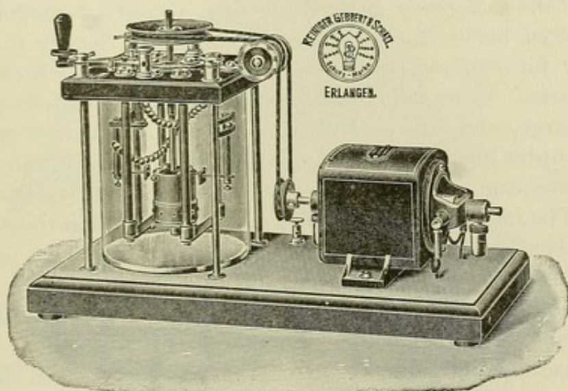
FIG. 71.—Mercury interrupter.
