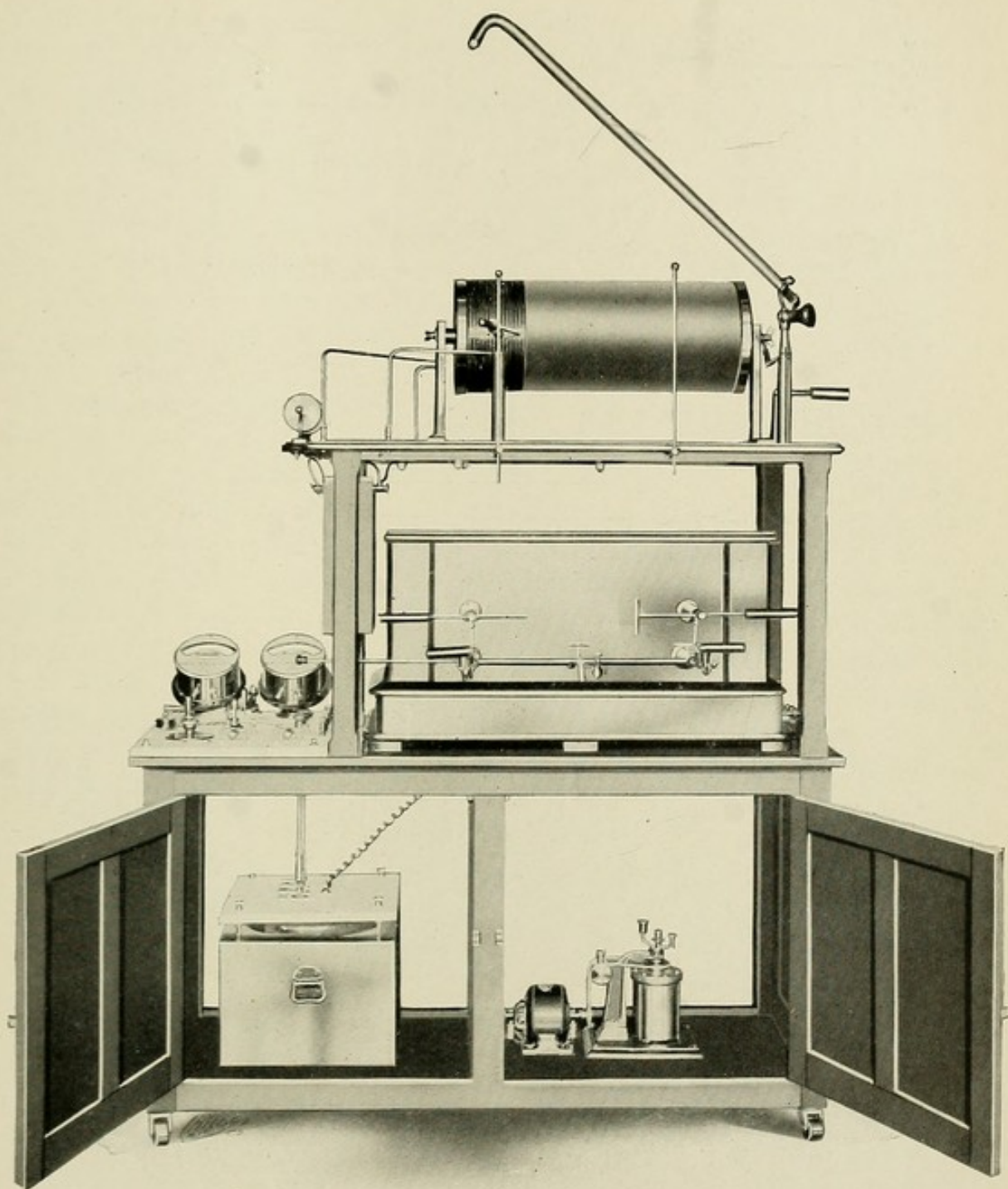
FIG. 81A.—Scheidel-Western coil combination radiographic special and high-frequency outfit for alternating or direct current.
