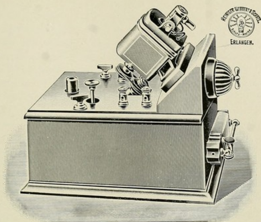
FIG. 72.—Davidson's interrupter.
