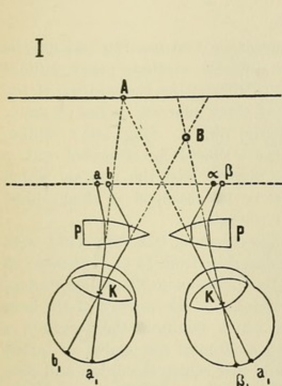
FIG. 110.—Principles of Brewster's refracting stereoscope.
