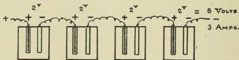
FIG. 2.—Connection of the cells in "series."
