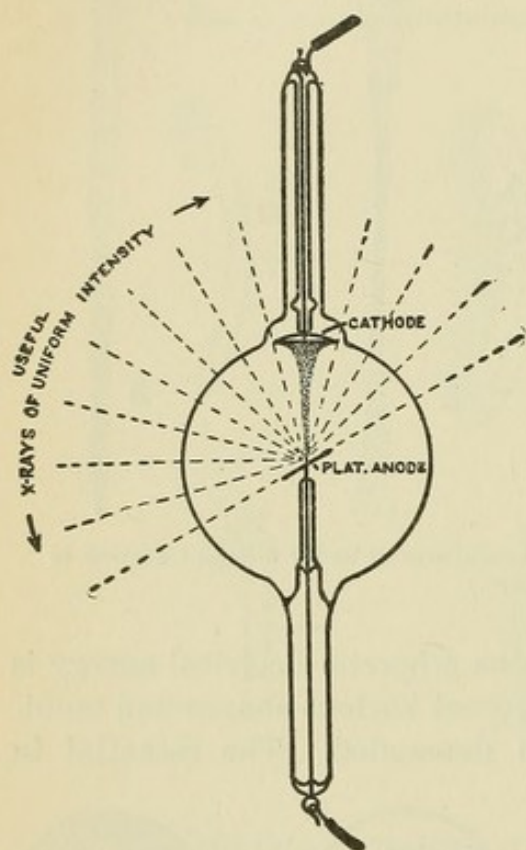
FIG. 88.—Essential features of an X-ray tube.
