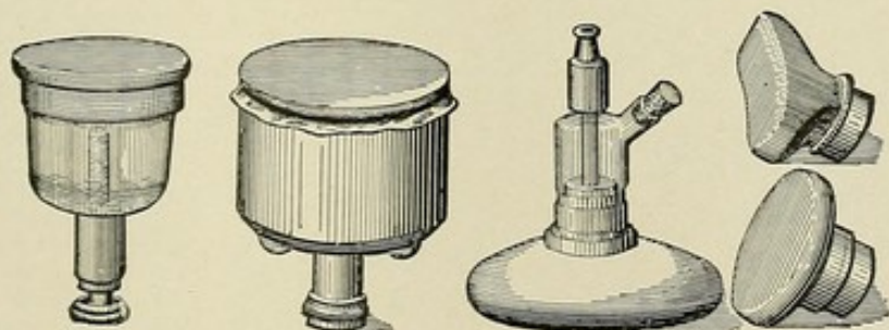
FIG. 30B.—Three varieties of cataphoric electrodes.
