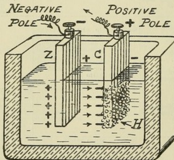
FIG. 23.—Galvanic cell.
