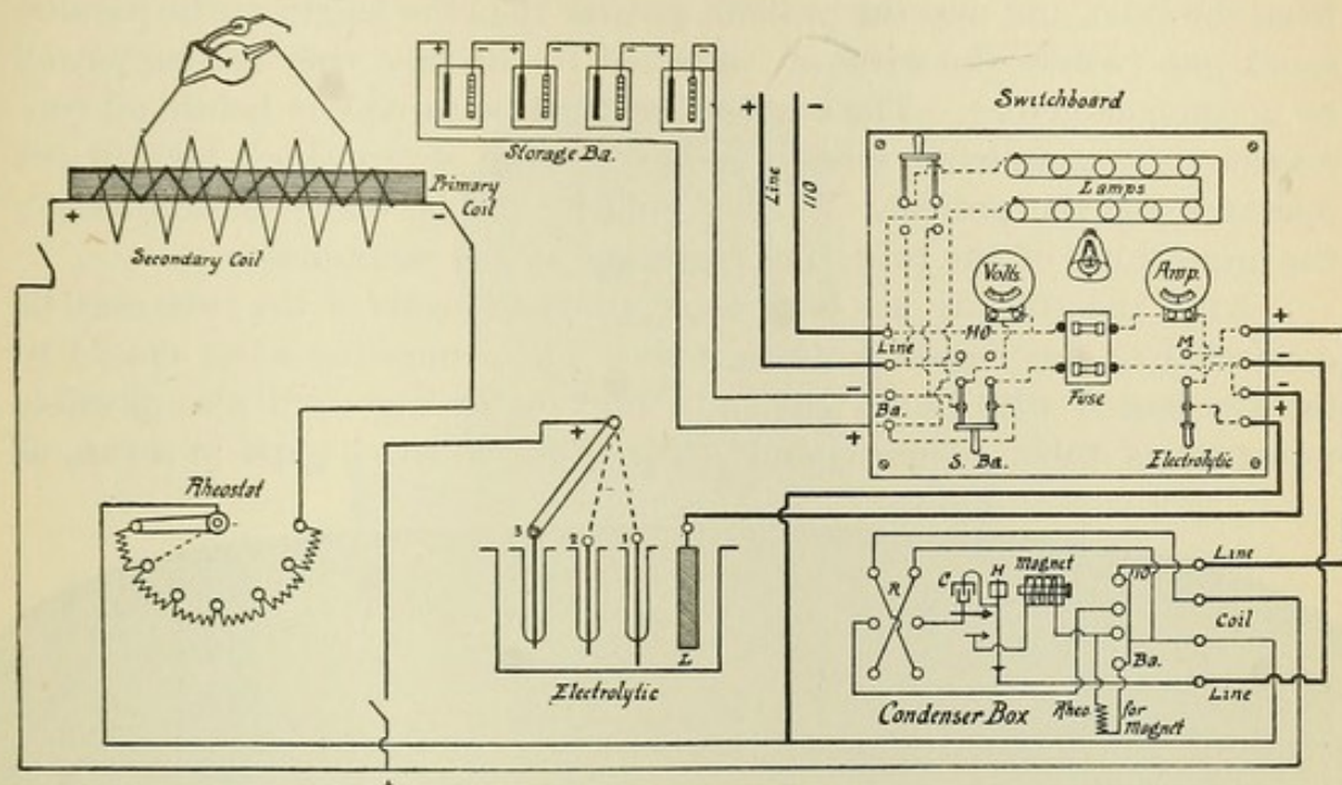
FIG. 102.—Author's office outfit.
