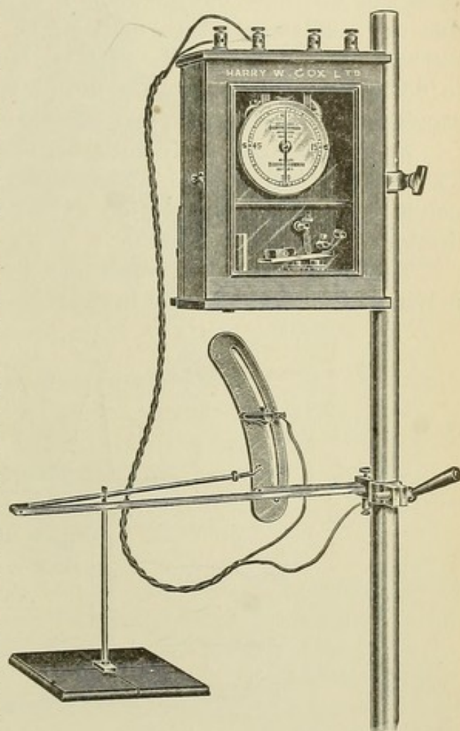
FIG. 191.—Clock arrangement and break of the same.
