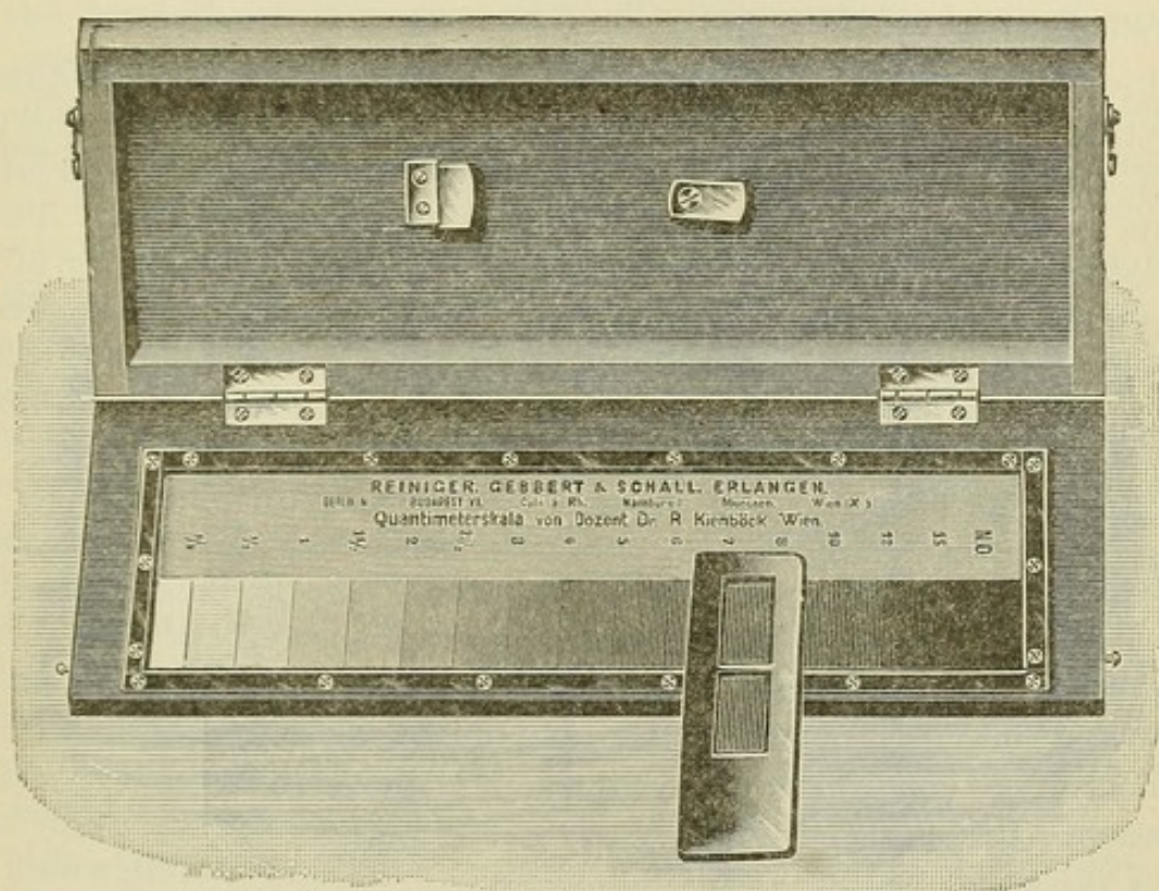
FIG. 221.—Kienböck's quantimeter.
