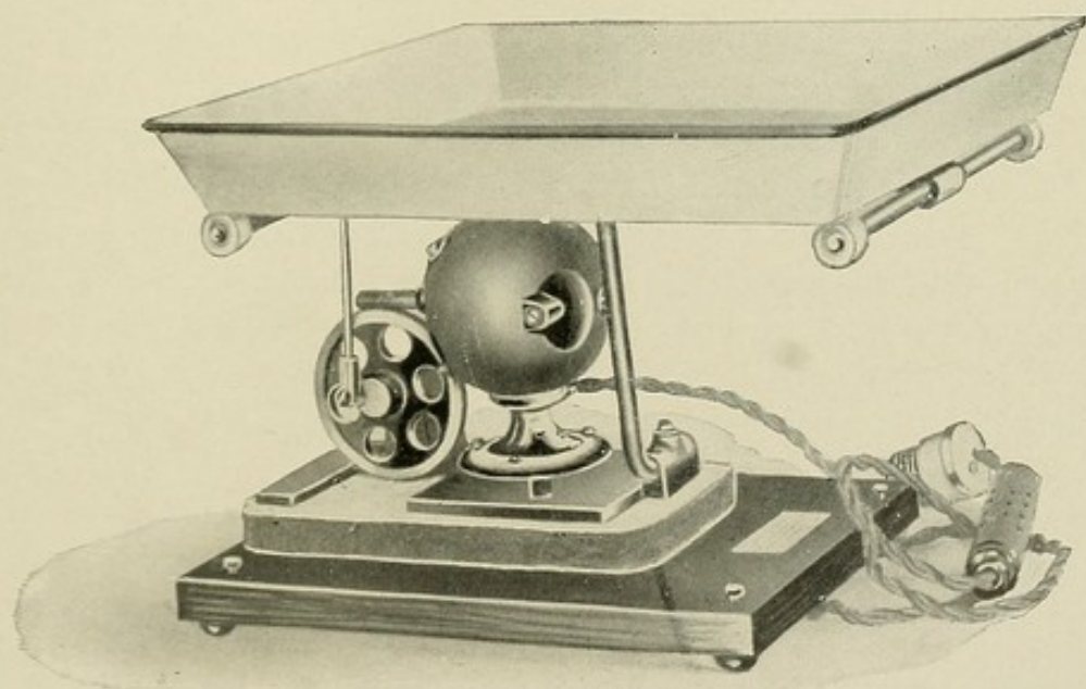
FIG. 107.—Automatic tray-rocker. (Röntgen Manufacturing Co.)
