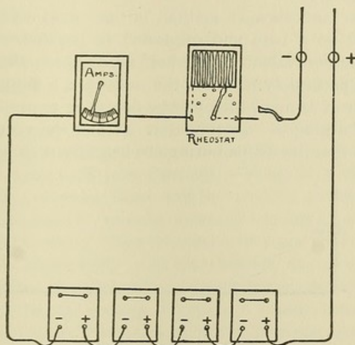
FIG. 6.—Diagrammatic view, illustrating the charging of a battery by the ammeter and volt-meter.
