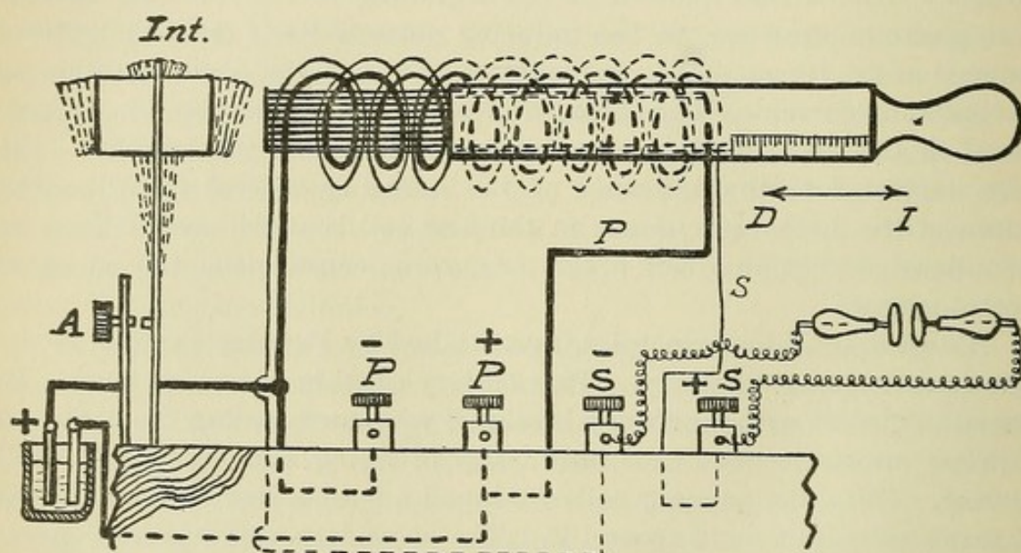
FIG. 28.—Medical induction coil.
