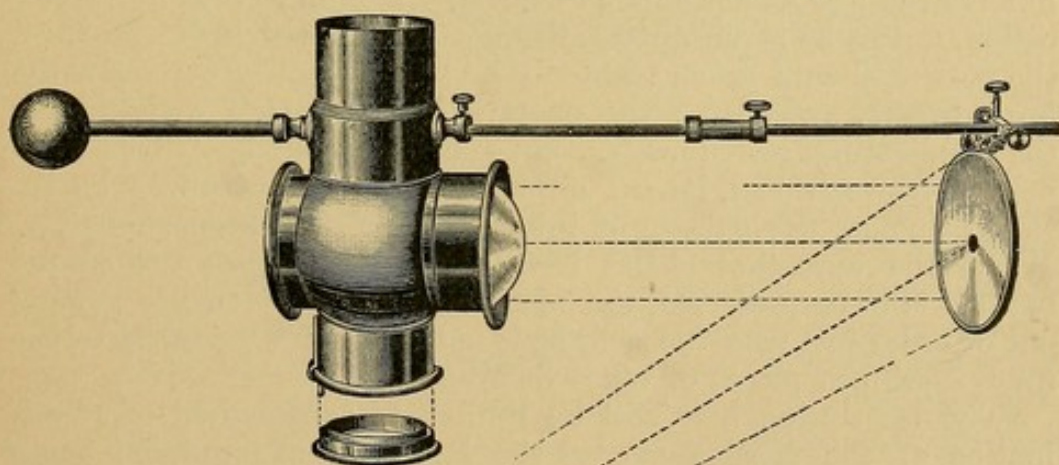
FIG. 13.—Mackenzie condenser and reflecting mirror.
