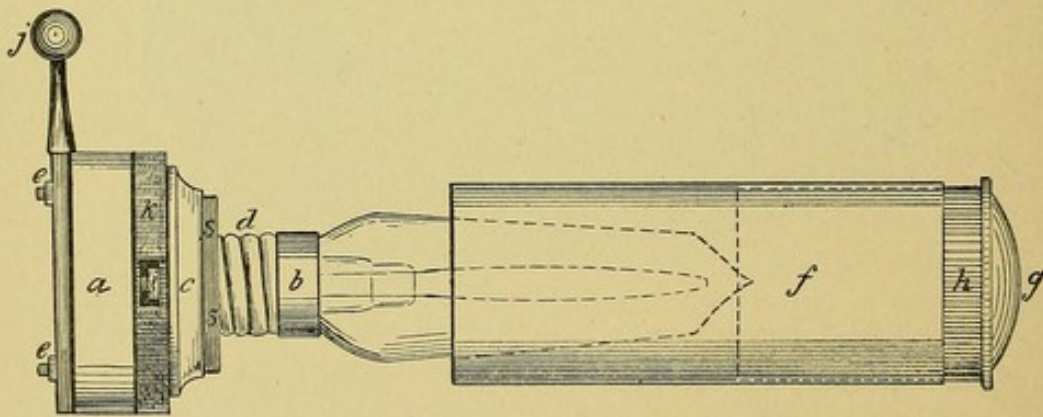
FIG. 11.—Gleason's electric head-lamp.
