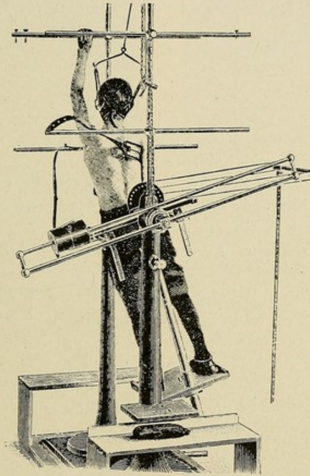
FIG. 81.—HIP-PENDULUM AND SHOULDER-RAISING APPARATUS.—(Schulthess.)
