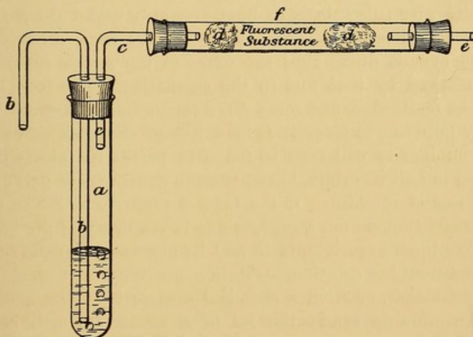
FIG. 28.—Apparatus for observing the connection. a is a test tube, containing radium solution. This tube is closed by a cork with two holes admitting two smaller tubes. One of these, b , passes to the bottom of the tube. The other, c , only just enters it. c is connected by means of another cork to the wider tube, f . f contains the fluorescent substance, confined between plies of cotton wool, d , d . A small exit tube, e , is fitted to f by a cork.
