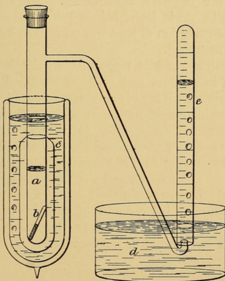
FIG. 26.—Measurement of the heat emission of radium at the temperature of liquid air or liquid hydrogen. A double-walled vessel, a (vacuum jacketed), contains the liquid hydrogen. The radium, b , in a sealed tube, is immersed in this, and causes ebullition. The evolved gas is collected over water in d , in a graduated tube, e . To prevent the access of external heat, a is immersed in an outer vessel, c , also containing liquid hydrogen.
