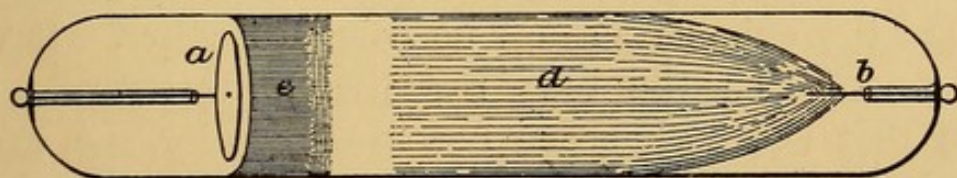
FIG. 1.—Electric discharge at a moderately low pressure. The negative electrode a is a disk, and is separated by a small dark interval from the blue negative glow e . The glow along the rest of the tube to the anode b is, in air, a diffuse band of reddish light, d .
