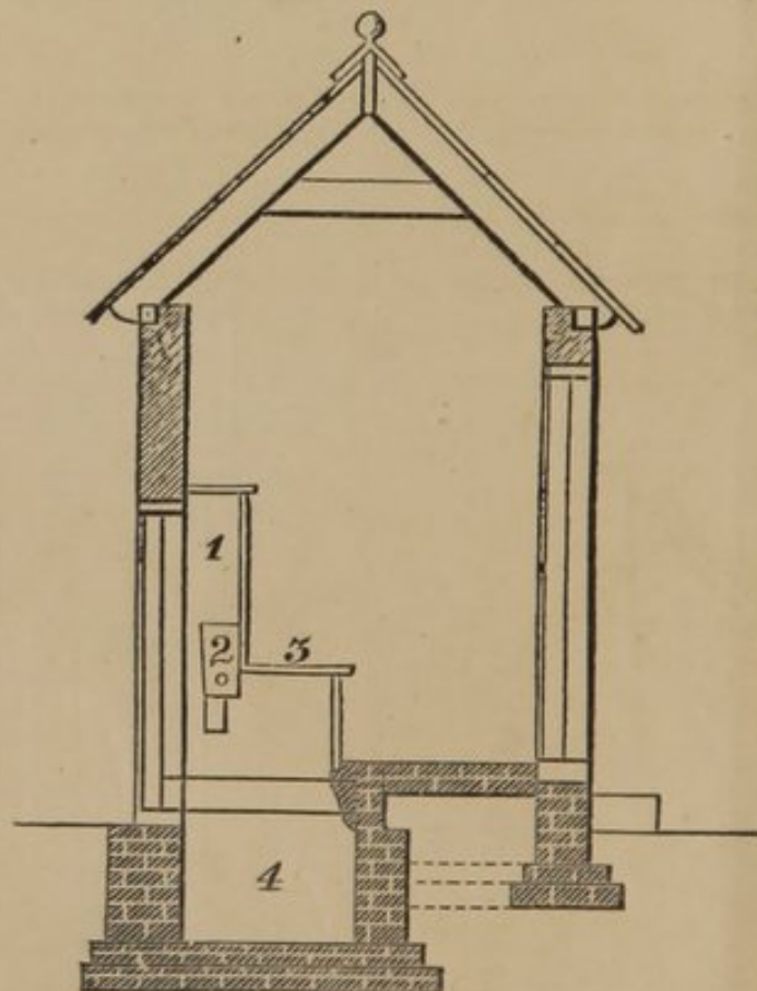
FIG. 7.—LONGITUDINAL SECTION.
