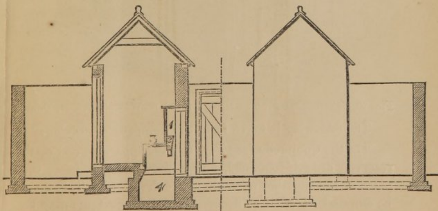
FIG. 9.—SECTION ON LINE. A, B.
