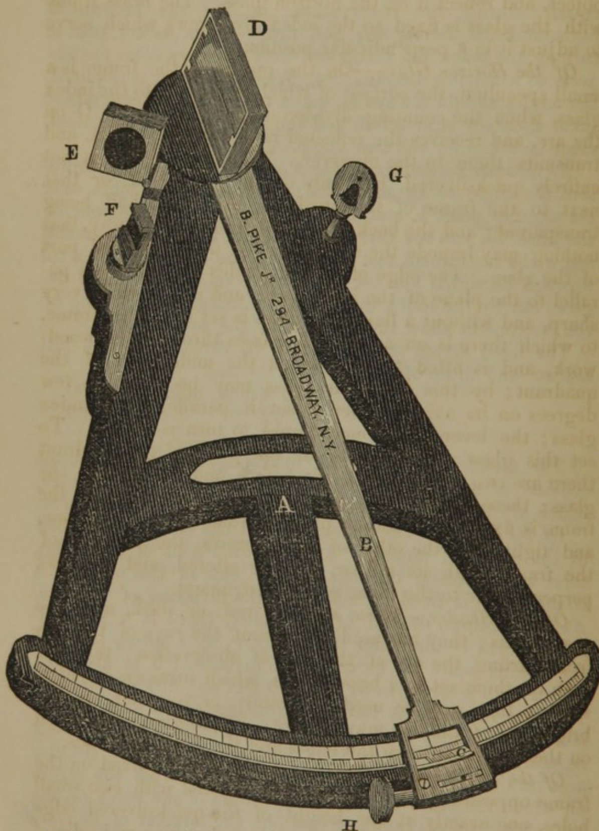
A. Frame and arc; B. Index; C. Nonius scale; D. Index glass; E. Dark glasses or screens; F. Horizon glass; G. Vane or sight
