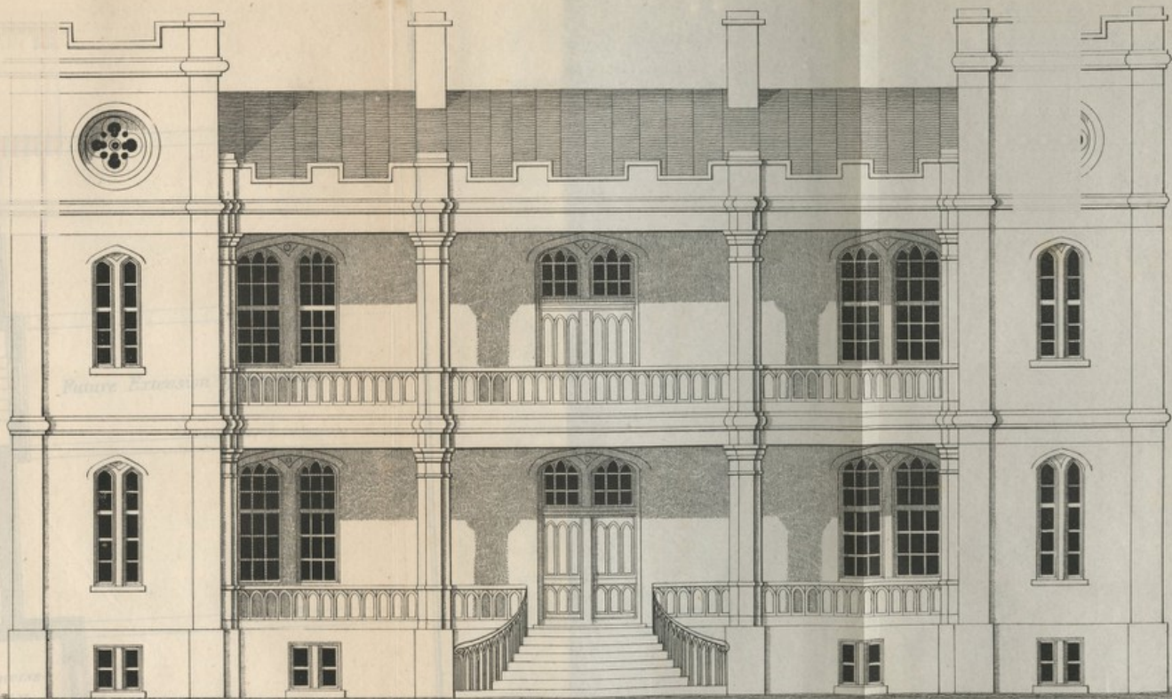
FACADES OF MARINE HOSPITAL TO ACCOMMODATE 50 PATIENTS BESIDES OFFICERS ROOMS &C.
