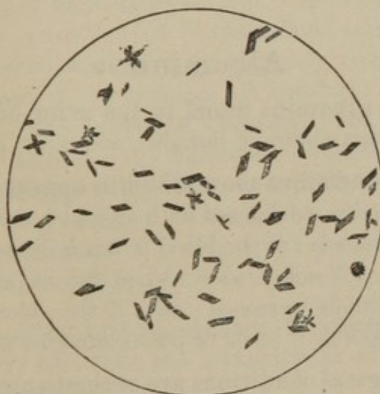
Teichmann's Hæmin Crystals.
