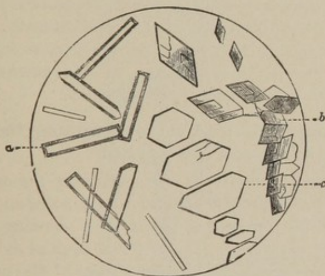
a, urea; b, rhombic, and c, hexagonal plates of urea nitrate.
