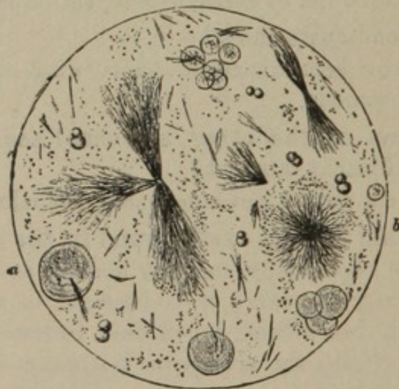
(a) Leucin, spheres; (b) Tyrosin, needles and sheaves.
