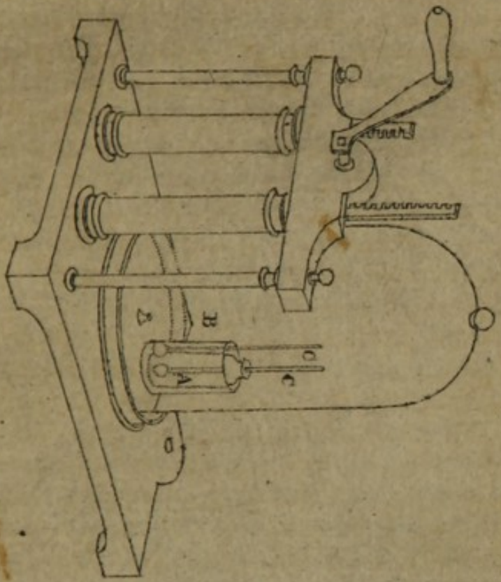
Pneumatic Pump
