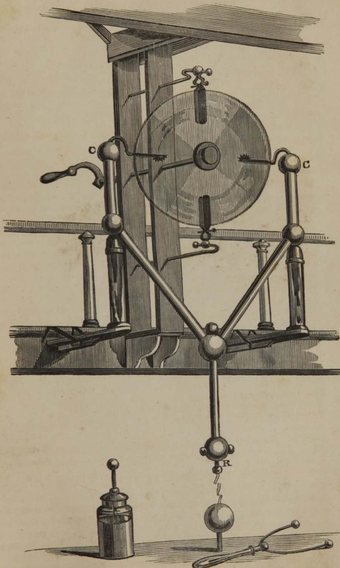
Large Electrical Plate Machine. (E. p. 7.)
