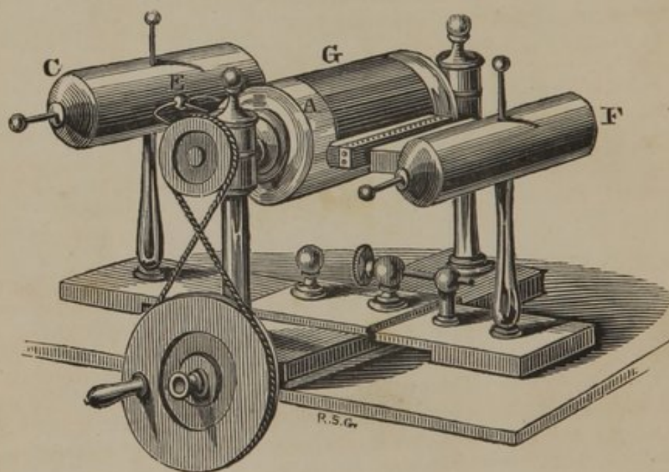
Electrical Cylinder Machine. (E. p. 7.)
