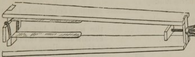
Crandall's apparatus complete. The counter-extending straps are passed over a block of wood supported above the knee, to prevent their pressure upon the sides of the knee.
