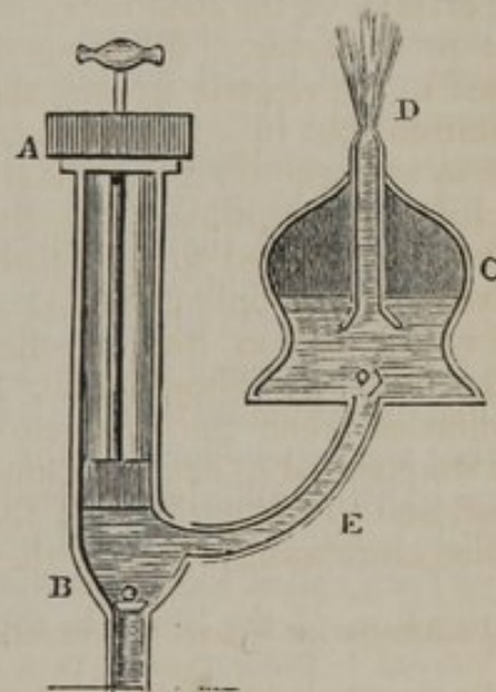
Section of a Forcing Pump.
