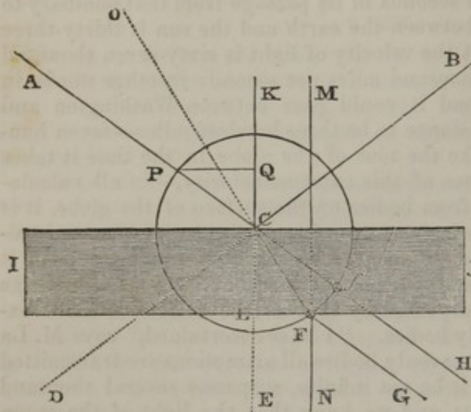
Reflection and Refraction of Light.
