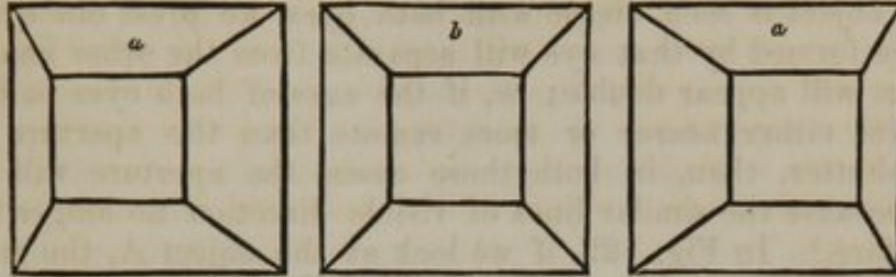
Binocular Vision.—Professor Wheatstone's Experiment.
