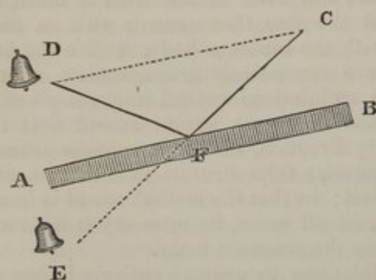
Reflection of Sound.
