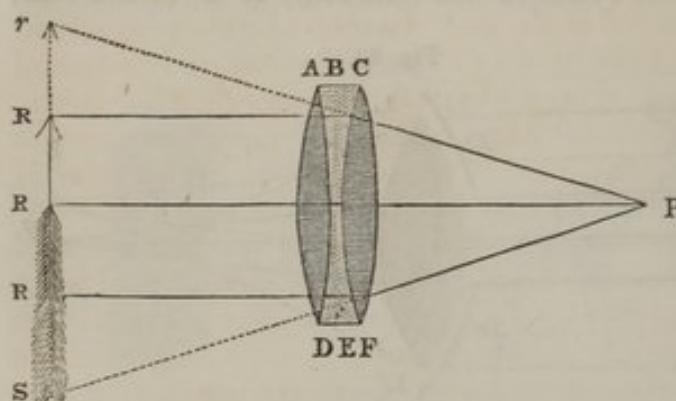
Aberration of Refrangibility.
