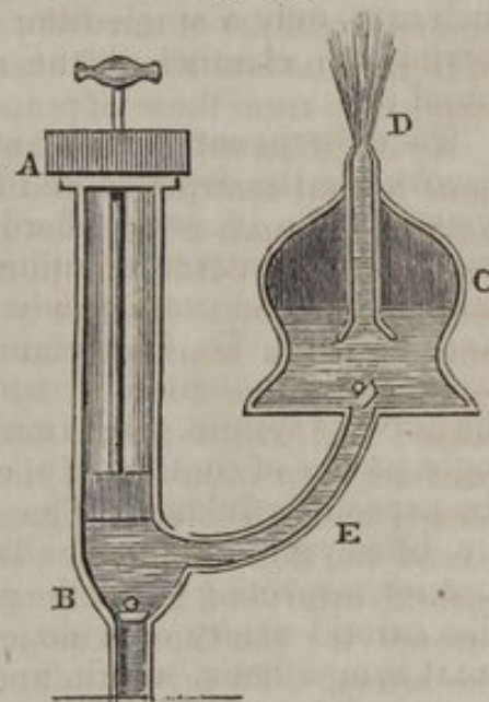
Section of a Forcing Pump.
