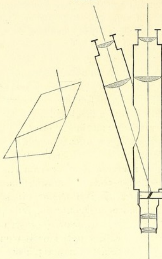
Wenham's Prism for the Binocular Microscope.
