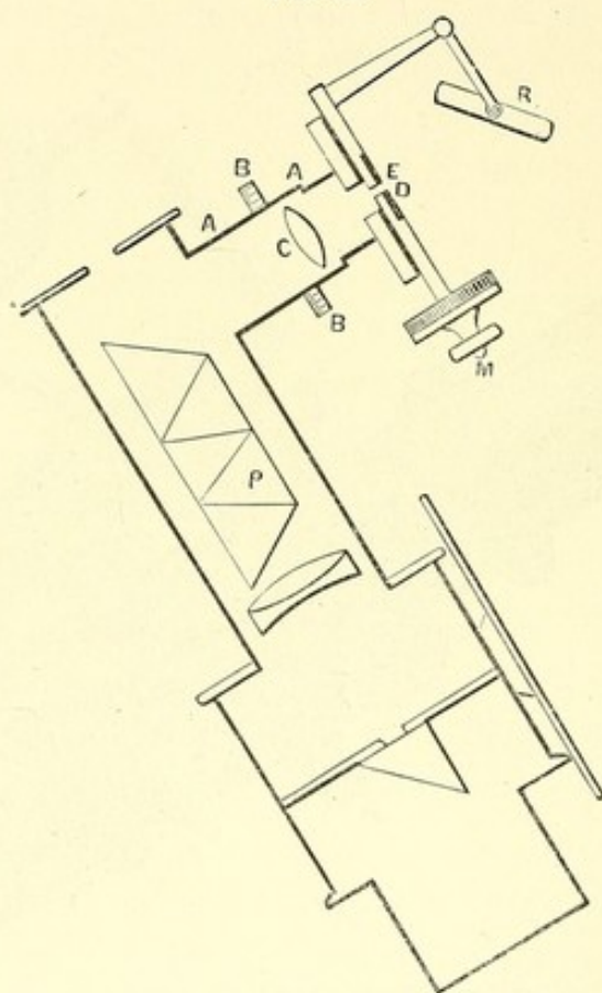
Spectroscope with Micrometer.
