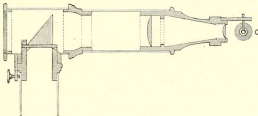
Oberhauser's Drawing Apparatus.
