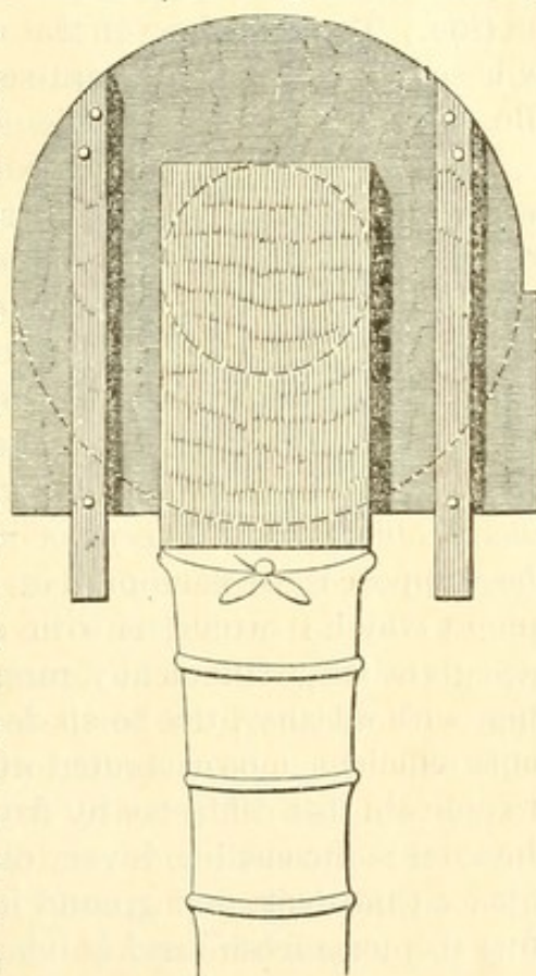
No. 12.—Fan for ventilation.
