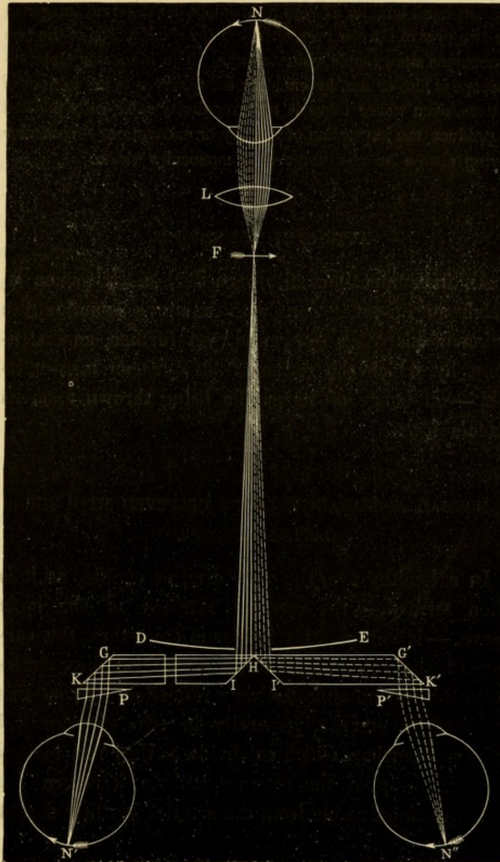
Fig. 10. The Binocular Ophthalmoscope.
