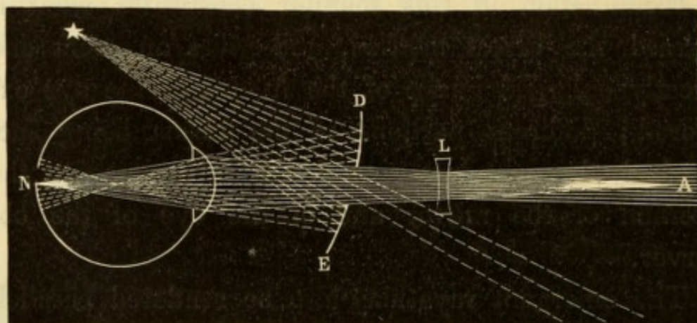
Fig. 4. Ophthalmoscope, with concave metallic or silvered glass mirror, showing greater extent of illumination; also showing the use of a concave eye-glass.
