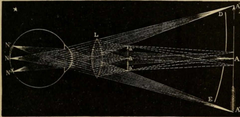
Fig. 6. Ophthalmoscope with concave mirror and convex objective lens, showing the formation of an inverted image. The illuminating rays are omitted.
