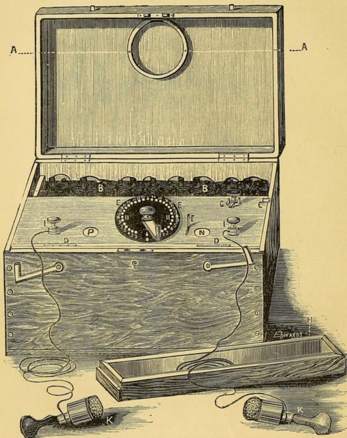
40-Cell Voltaic Battery.
