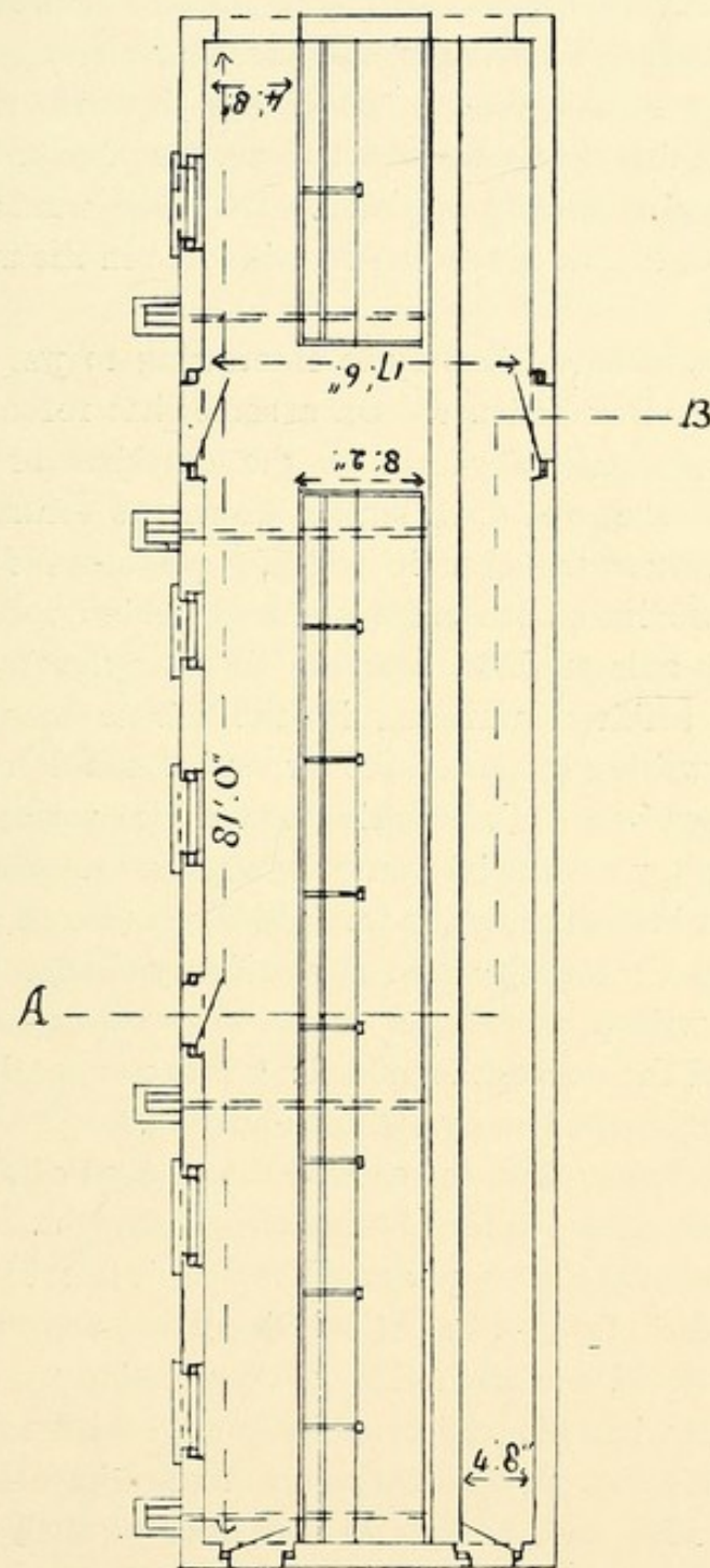
GROUND PLAN OF COWSHED.
