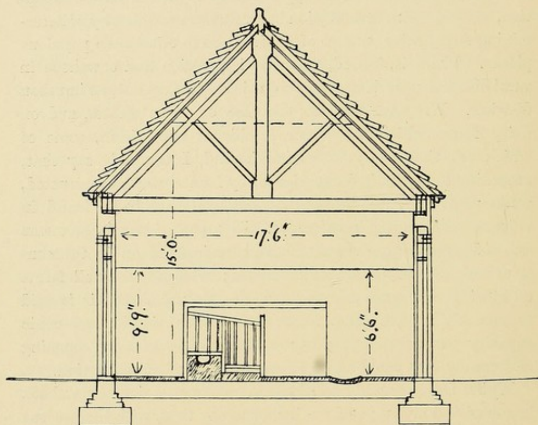
SECTION OF COWSHED.
