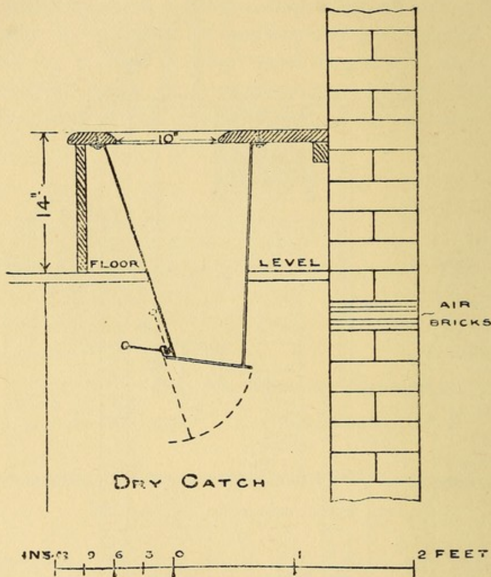
FIG. 19.—SECTION OF PAN FOR DRY CLOSETS.
