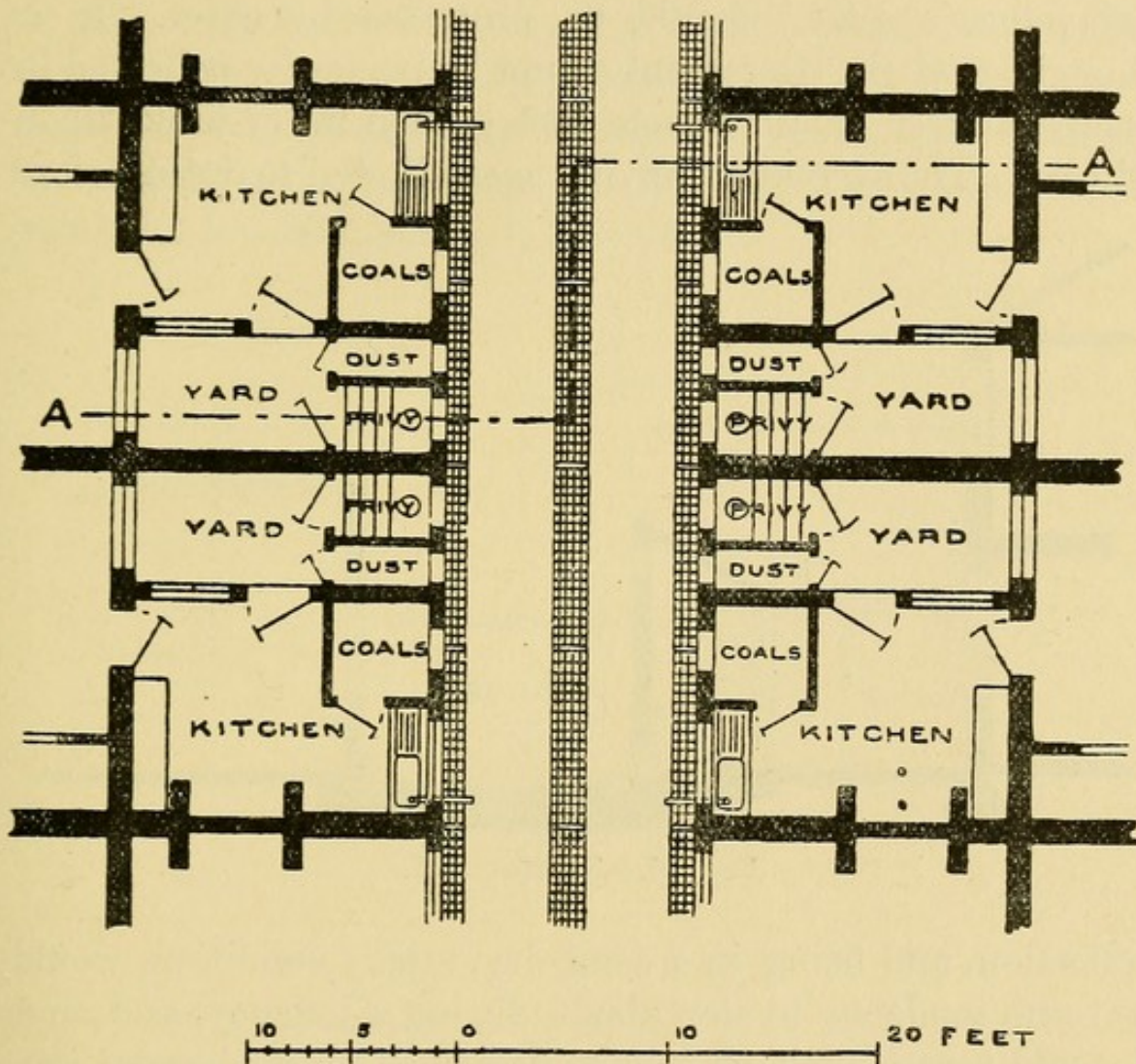
FIG. 29.—ARRANGEMENT FOR SMALL TENEMENTS.
