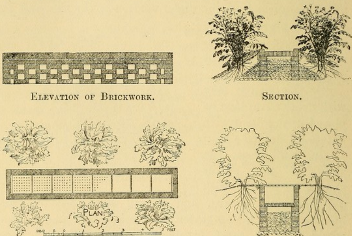
FIG. 27.—FILTRATION GUTTER ON BANK.
