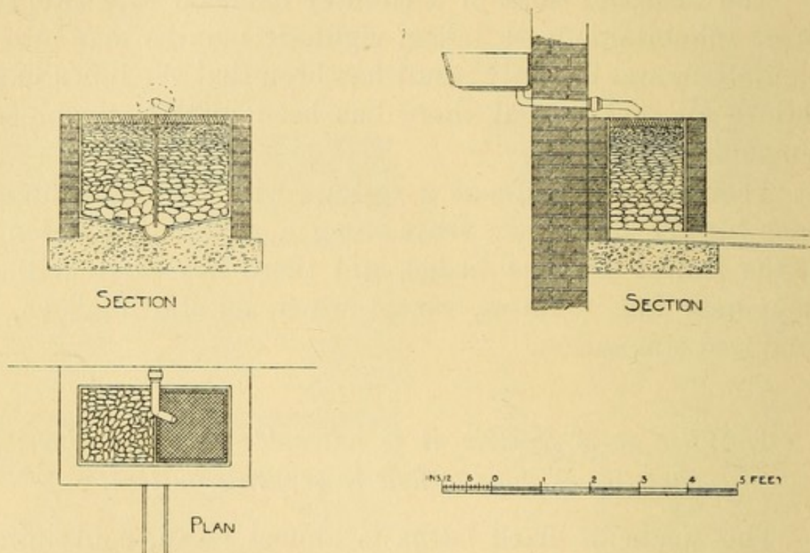
FIG. 28.—KITCHEN SINK WITH DUPLICATED OUTSIDE FILTER.
