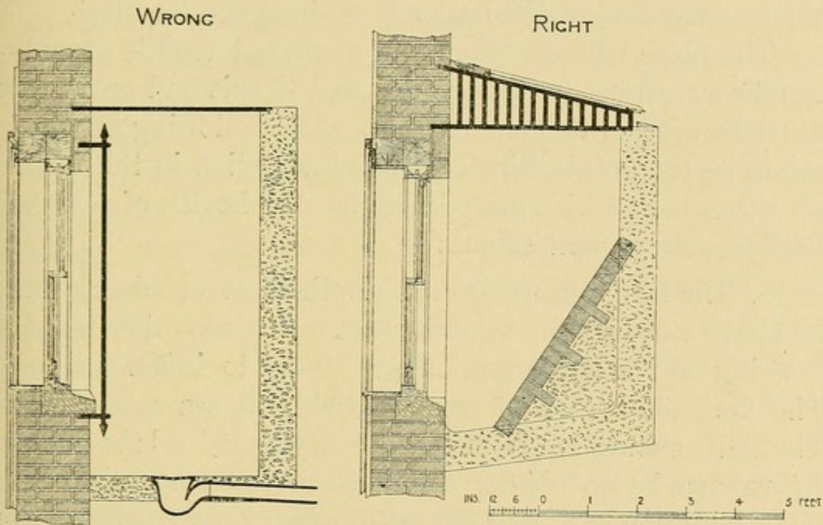
CELLAR WINDOW.
