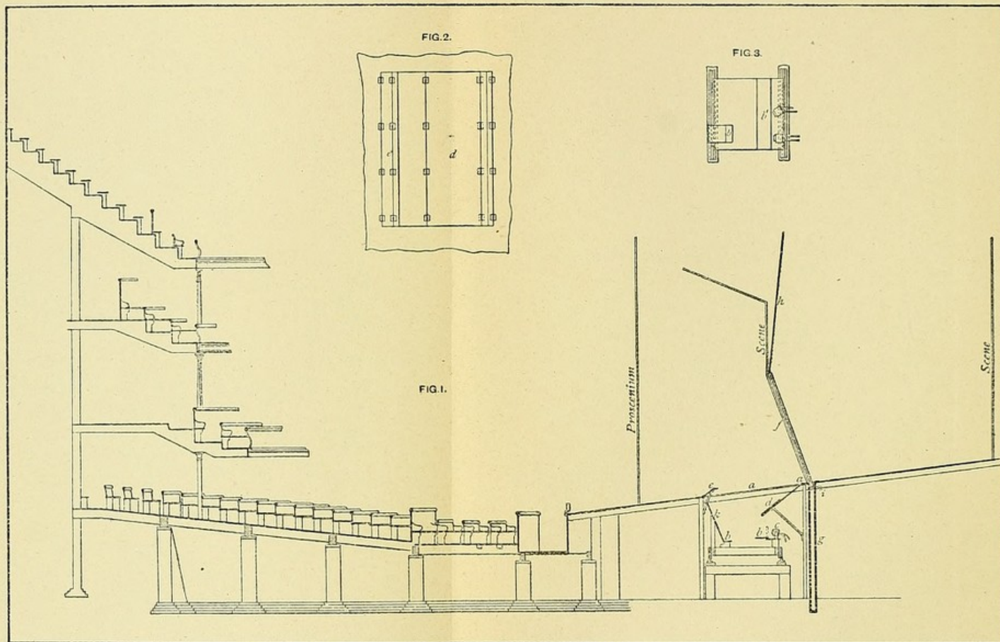
DIAGRAMS ILLUSTRATING THE "GHOST" MACHINERY. (See p. 8.) (From a drawing by Mr. Barnard Chalon.)
