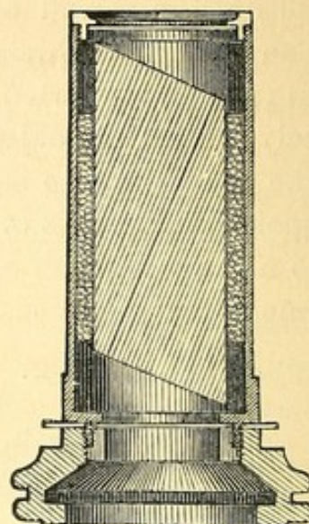
SECTION OF ANALYZER.
