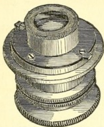
MOUNTING OF POLARIZING PRISM.
