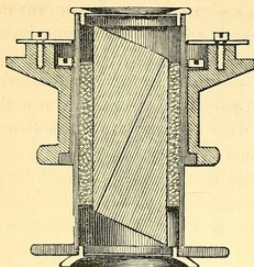
SECTION OF POLARIZER.
