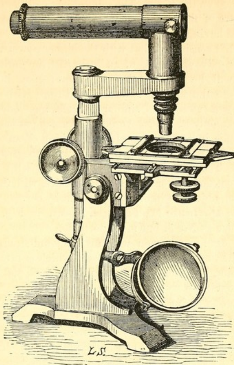
CHEVALIER'S PRISMATIC BODY, AND BAILEY'S INDICATOR STAGE.
