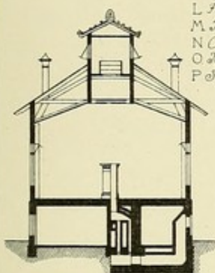
half transverse & longitudinal Section thro Pavilions
