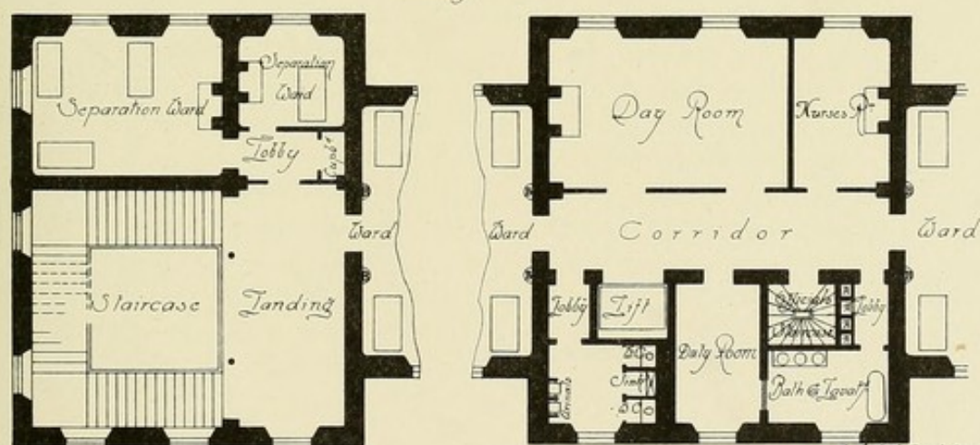
R. Fresh air Sale's Price :Detail:of:one:of:End:Blocks: :Detail:of:Central:Block:
