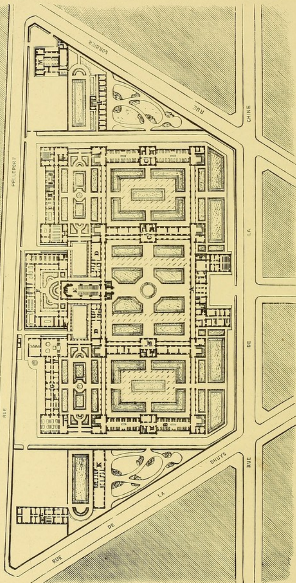
GENERAL PLAN OF THE MENILMONTANT HOSPITAL.
