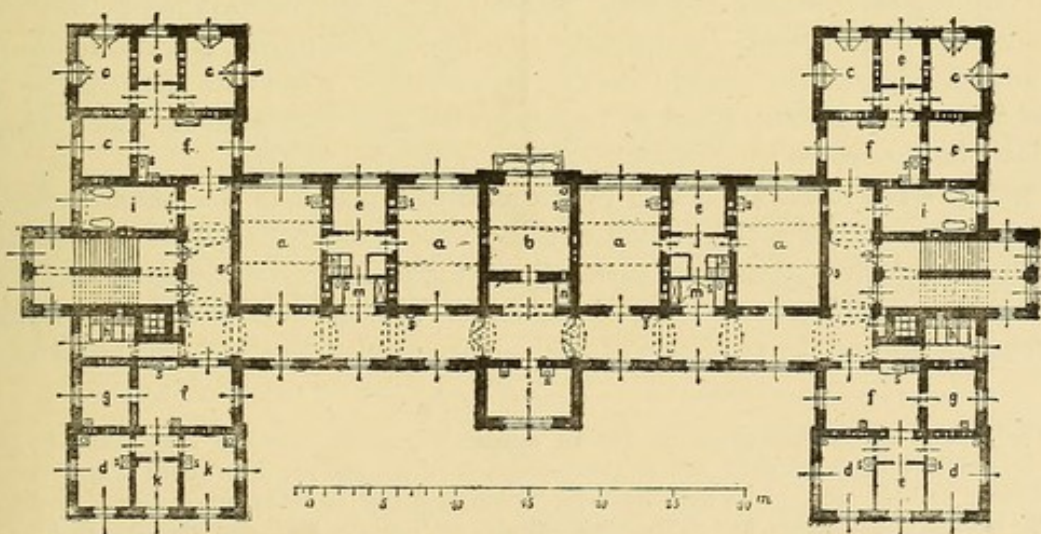
GROUND PLAN OF MUTTERHAUS.
