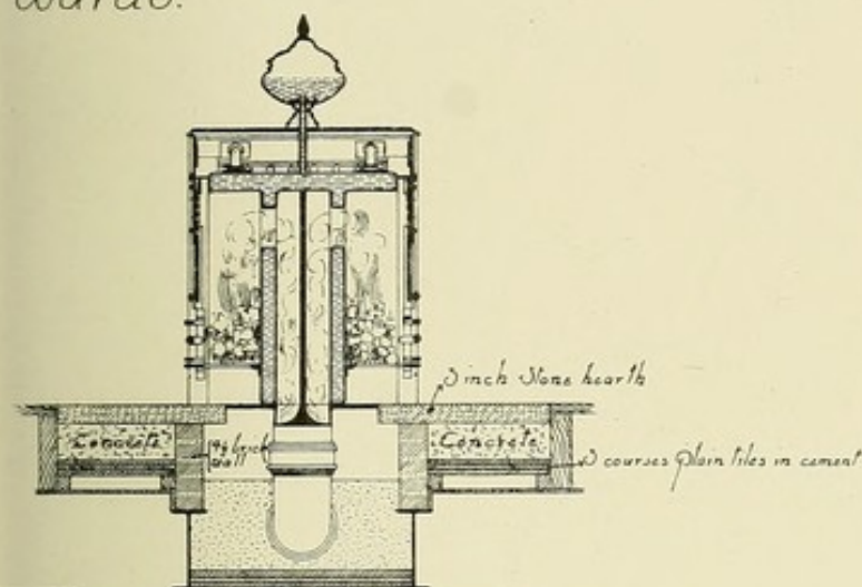
Section thro Stove B.B
