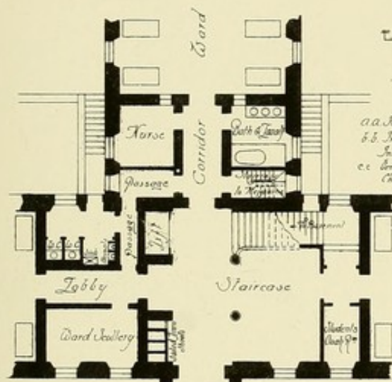
:Detail:of:Offices:
