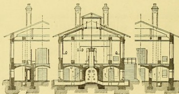
TRANVERSE SECTION THROUGH PAVILIONS.
