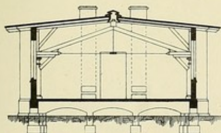
Section thro Medical & Isolation Wards
