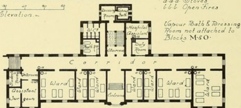
Ground Plan of Blocks L.M.N.O
