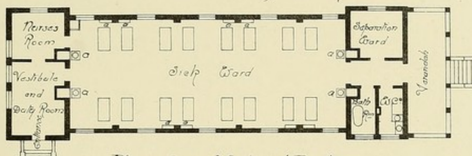
Plan of one Medical Pavilion
