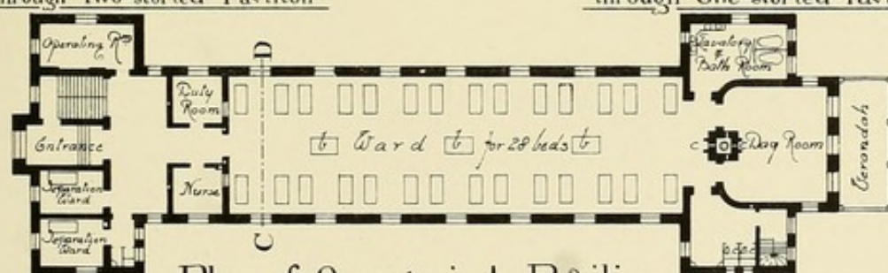
· Plan of One-storied Pavilion ·
