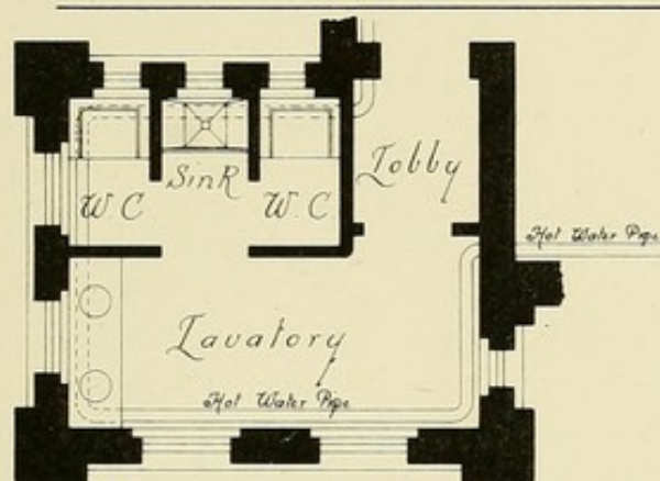
Plan of W.C.s · Scale of Feet · Section on line A.B.
