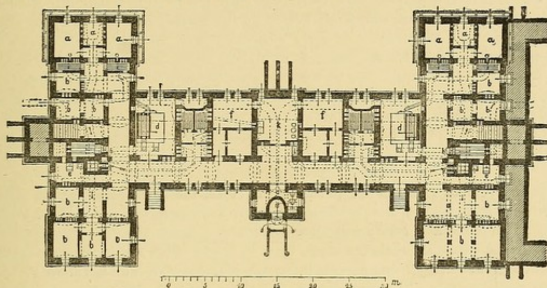
BASEMENT PLAN OF MUTTERHAUS.
