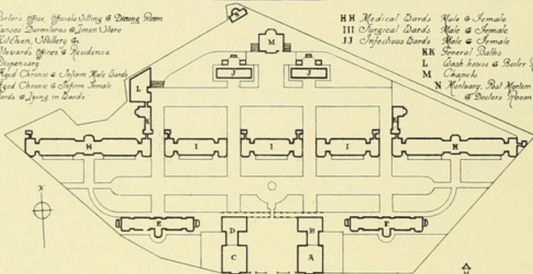
:Plan:of:Site:
