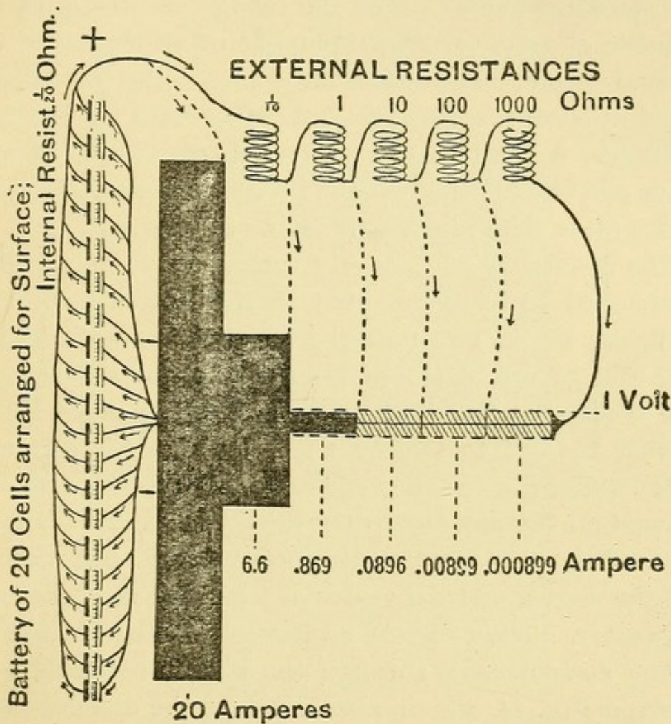
FIG. 43.—GRAPHIC DELINEATION OF THE VOLUMES AND PRESSURE OF CURRENTS FROM A BATTERY OF TWENTY CELLS ARRANGED FOR "SURFACE."—The battery, acting as an enlarged cell, has an electromotive pressure of one volt and an internal resistance of one-twentieth of an ohm. The first three imaginary current sections show the proportions of volume to the eye.
