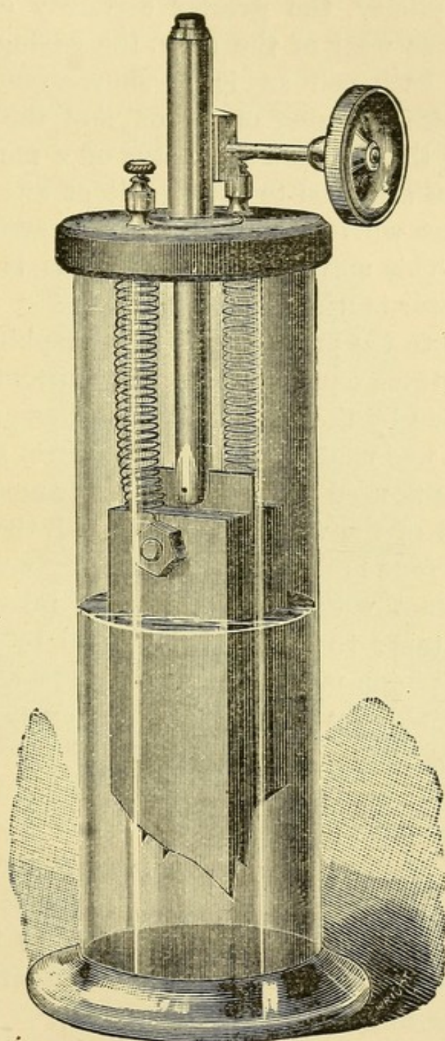
FIG. 4.—BAILEY CURRENT CONTROLLER.
