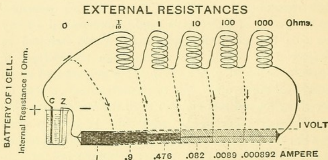
FIG. 42. — GRAPHIC DELINEATION OF THE VOLUMES AND PRESSURE OF CURRENTS FROM A SINGLE GALVANIC CELL WHEN VARIOUS RESISTANCES ARE INSERTED INTO THE EXTERNAL CIRCUIT.—The cell shown at the left of the cut has an electro-motive pressure of one volt and an internal resistance of one ohm. The divisions of the drawing to the right of the cell represent imaginary longitudinal sections of the currents obtained on short-circuiting the cell and after successively inserting into the circuit the several resistance coils indicated in the upper portion of the figure. The heavy shading in the first three divisions shows the exact proportion of volume to the eye as compared with a full ampère, indicated by a broken line. The light shading shows the proportion of pressure, which is uniformly maintained throughout. The volume in the last three spaces is indicated by the figures beneath, but is much too small to be shown to the eye on the scale adopted.
