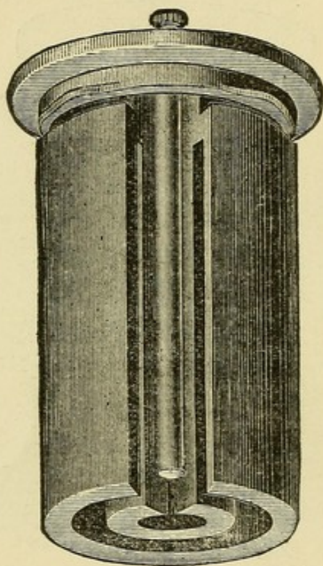
FIG. 2.—ELEMENTS OF THE LAW CELL.
