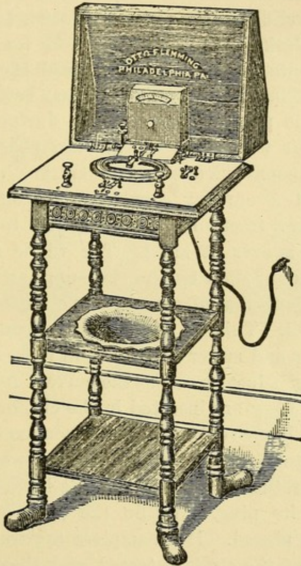
FIG. 8.—BEDSIDE GALVANIC TABLE.—For use with supply wires from an incandescent plant or permanent battery. Connection with the supply wires is made by a double plug and socket, or by two binding posts.
