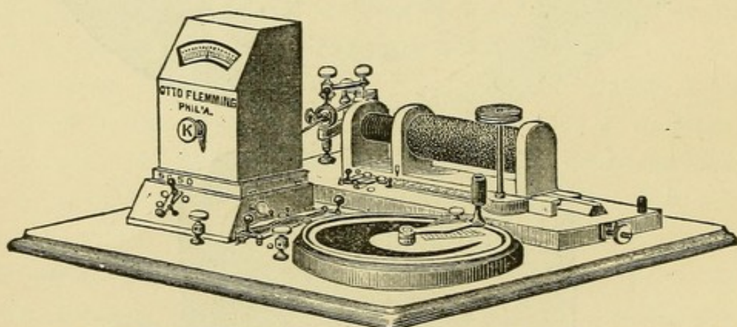
FIG. 7.—COMPLETE ELECTRO-GYNECOLOGICAL APPARATUS FOR BOTH CURRENTS. (Author's design.).—The faradic apparatus may be removed from the table when delicate galvanic measurements are made. Designed for incandescent current or cells.
