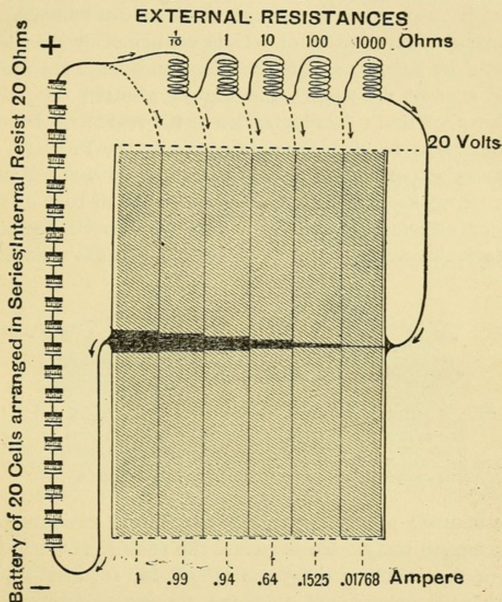
FIG. 41. — GRAPHIC DELINEATION OF THE VOLUMES AND PRESSURE OF CURRENTS FROM A BATTERY OF TWENTY CELLS ARRANGED IN "SERIES."—The battery has an electromotive pressure of twenty volts and an internal resistance of twenty ohms. The heavy shading in the first five imaginary current sections shows the exact proportion of volume on the scale of the preceding cuts. The space allotted to represent pressure is reduced to one-half the scale adopted in Figs. 42 and 43 for purposes of convenience.
