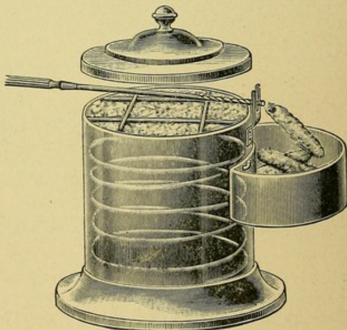
FIG. 17.—Cotton-reservoir and waste-box.
