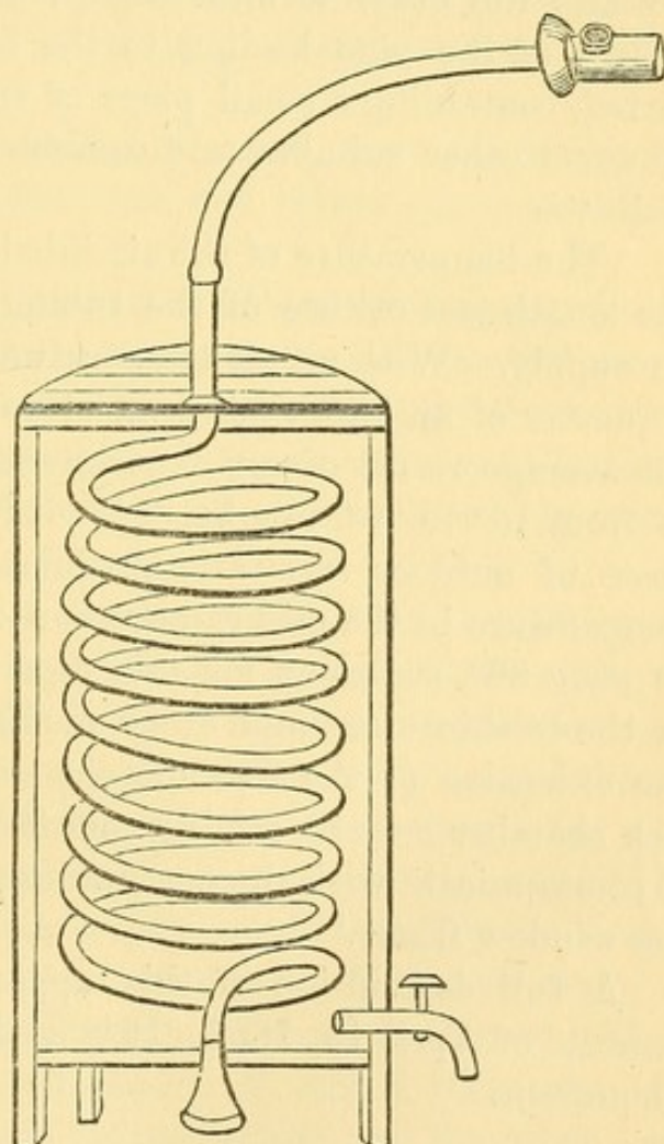
FIG. 1.—APPARATUS FOR COOLING THE AIR.
