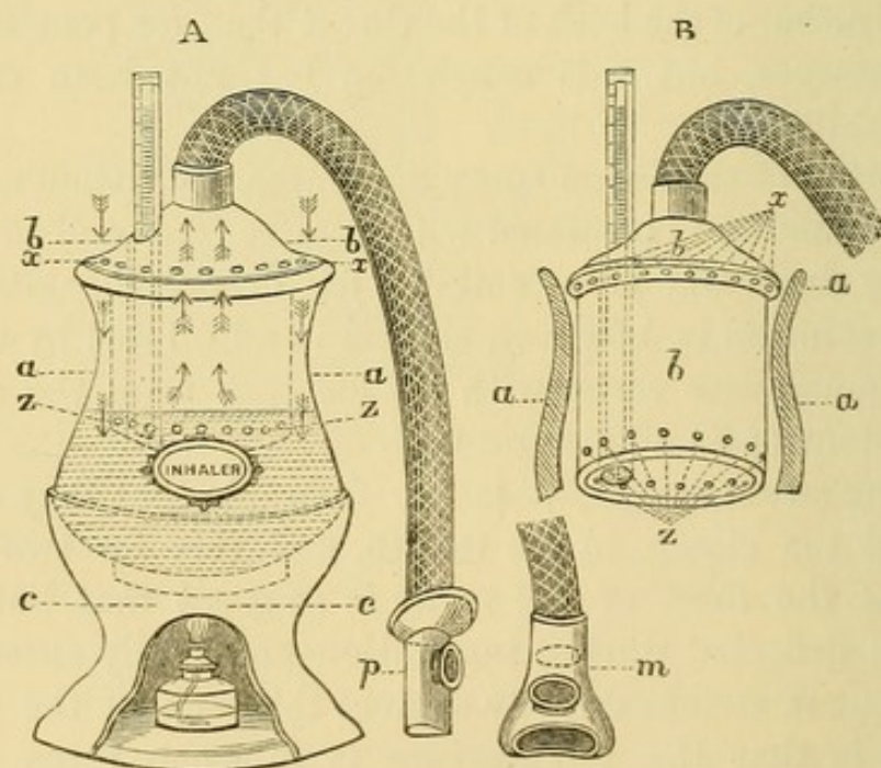
FIG. 13.—DR. MORELL MACKENZIE'S ECLECTIC INHALER.
