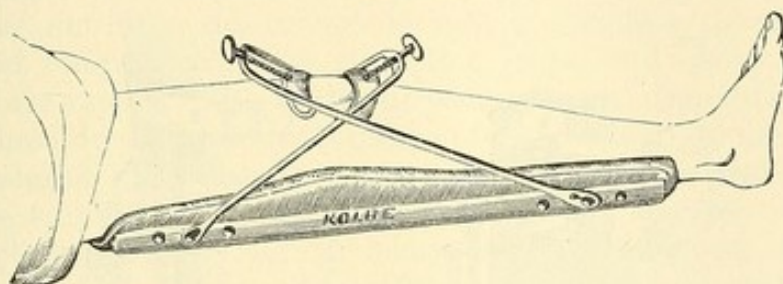
Lausdale's apparatus.
