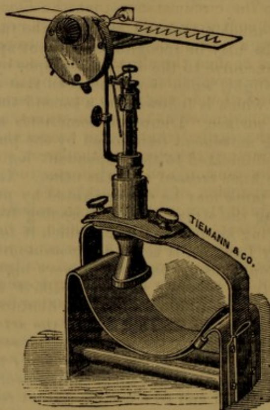
FIG. 37.—Pond's sphygmograph.
