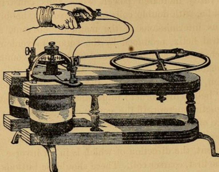
Fig. 66. Magneto-Electric Machine, showing its revolving Double Armature.
