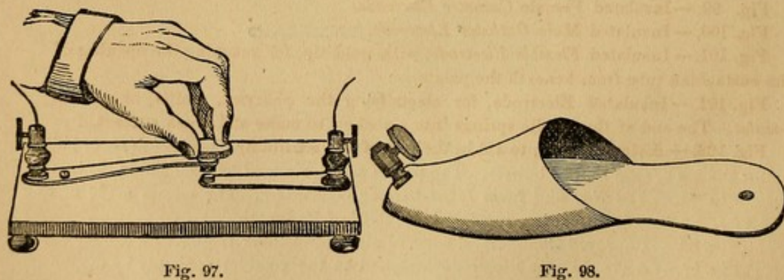
Fig. 97. — Foot-Board, or Current-Breaker, for dentists' use.
