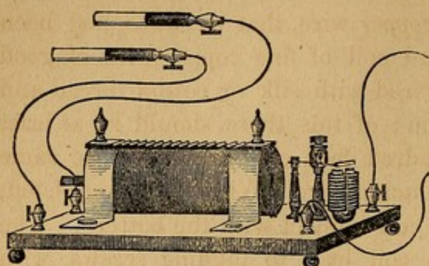
Fig. 51. Electro-magnetic Helix, with Vibrating Electrotome, but without its Battery.
