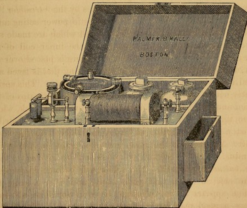
Fig. 53. Electro-Magnetic Portable Machine, complete in its Box.
