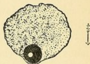
FIG. 23. — Section through the nucleus of a young ovum (1 mm. in diameter) showing the nucleolus, which has, apparently, caused a distention of the nuclear membrane by the pressure of its own weight. Arrow shows the direction of the earth's centre. Magnified 248 diameters. (From HERRICK, '95.)
