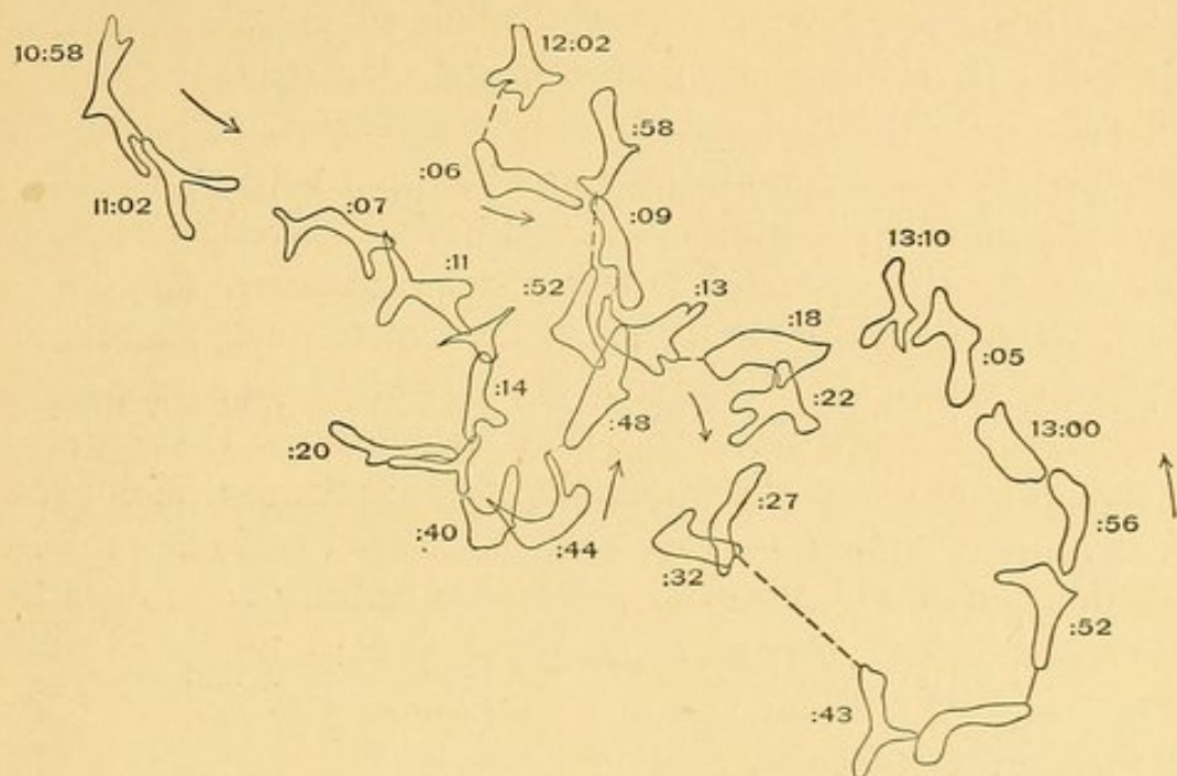
FIG. 72.—Camera drawing, showing the successive positions assumed by Amoeba proteus when acted upon by external agents uniformly in all directions. Magnified 16 diams.
