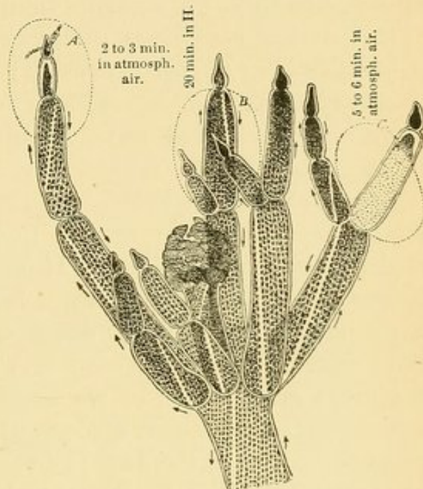
FIG. 49. — Piece of a sprout of Nitella mucronata which was subjected in a gas chamber to a green light in three successive experiments A, B, C. In experiment A the insolation lasted 2 to 3 minutes, the gas chamber being filled with atmospheric air. In experiment B the insolation lasted 20 minutes in the presence of hydrogen. In experiment C the insolation occurred again in the presence of atmospheric air and lasted 5 to 6 minutes. (From PRINGSHEIM, '81.)
