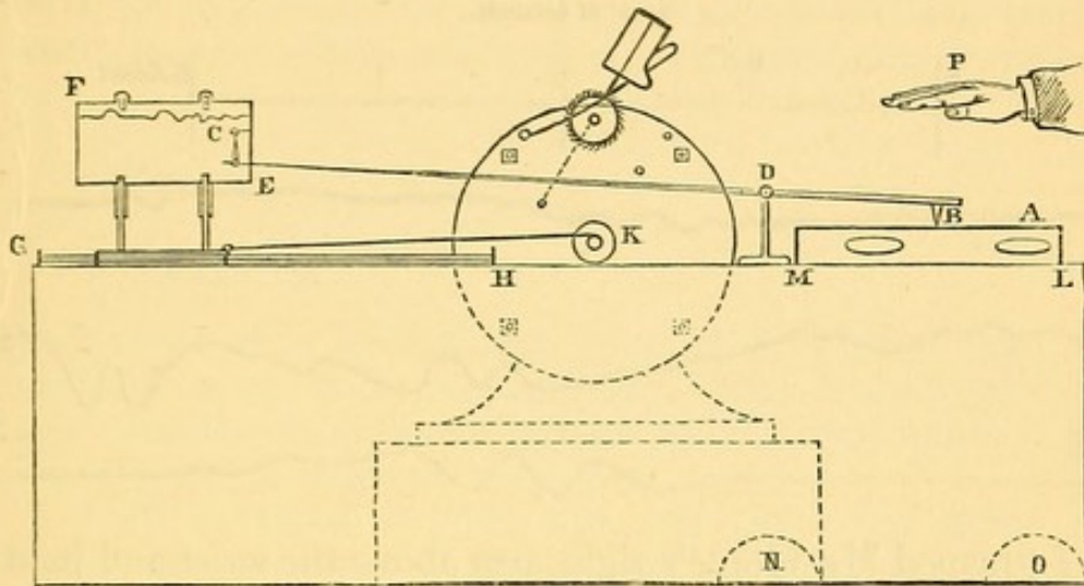
FIG. 10. (Section.)
