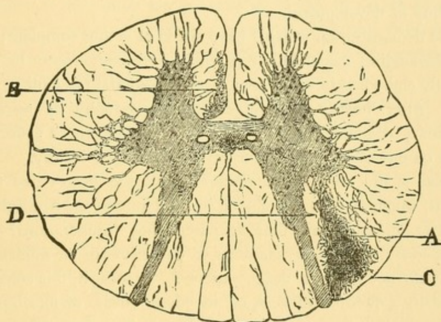
FIG. 13.—Transverse section of the cord in the cervical region. A, degeneration of the pyramidal fasciculus in a case of lesion of the hemisphere, motor centres. B, degeneration of the direct fasciculus. C, a space of white substance corresponding to the cerebellar fasciculus. D, region intermediary between the posterior horn and the pyramidal fasciculus; this region is always respected in descending degenerations.
