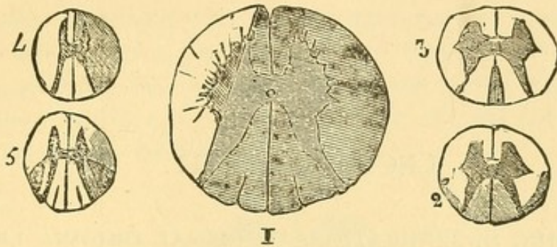
FIG. 20.—1, transverse section of the cord on the level of the fourth dorsal vertebra. The whole of the right half of the cord, and all the extent of the posterior columns are destroyed. 2, section of the cord on the level of the third dorsal vertebra (sclerosis of the two posterior columns and the two cerebellar fasciculi). 3, above, the degeneration occupies no more than the two columns of Goll. 4, the cord at the level of the sixth dorsal (degeneration of all of the antero-lateral columns). 5, lower down at the height of the seventh and eighth dorsal vertebrae the degeneration of the right lateral fasciculus is accompanied by a degeneration of the left pyramidal fasciculus.
