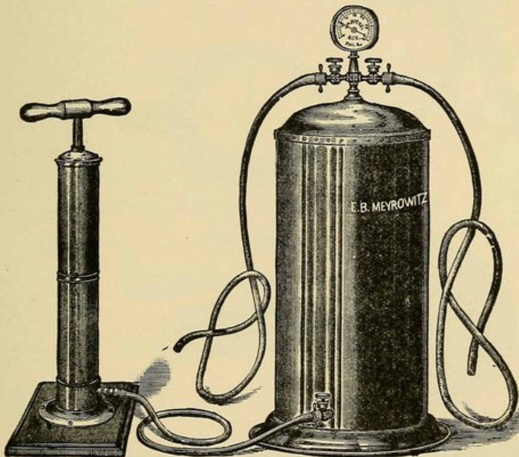
Fig. 27.—Compressed-air apparatus.
