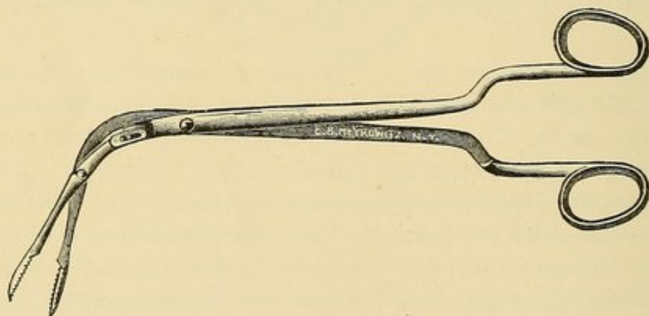
Fig. 139.—Laryngeal polypus-forceps, Waxham's.
