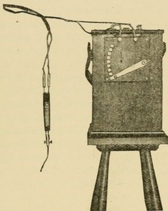
Fig. 47.—Ballard galvanocautery-battery, with cord, handle, and knife.
