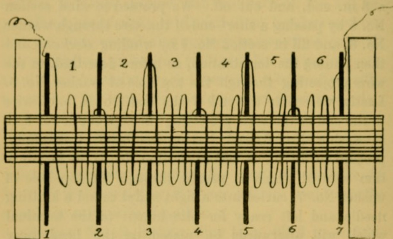
FIG. 6.—MODE OF WINDING SECTIONS.
