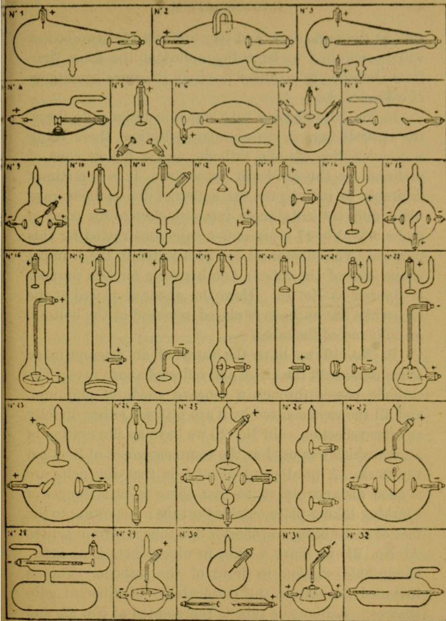
FIG. 22.—DIFFERENT FORMS OF CROOKES' TUBES.
