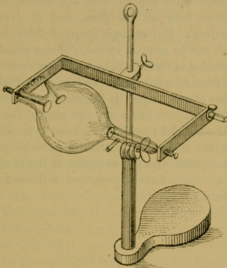
FIG. 24.—STAND FOR BIANODIC TUBE.
