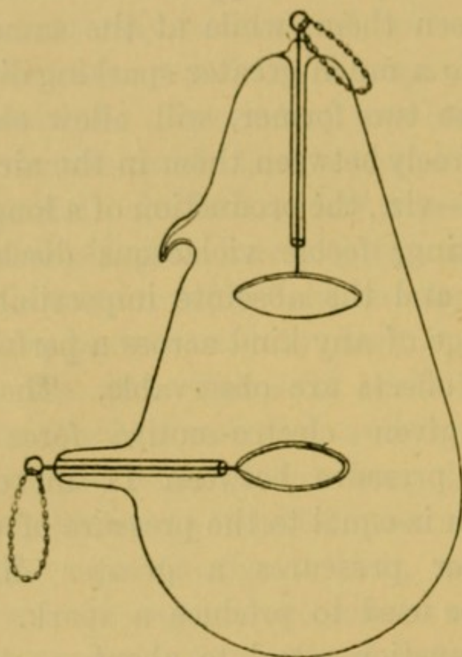
FIG. 2.—CROOKES' TUBE (OLD FORM).
