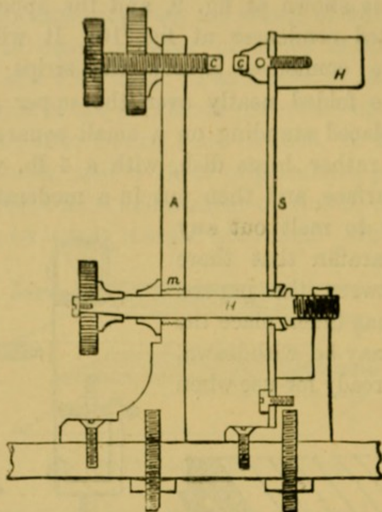
FIG. 12.—APPS' CONTACT-BREAKER.
