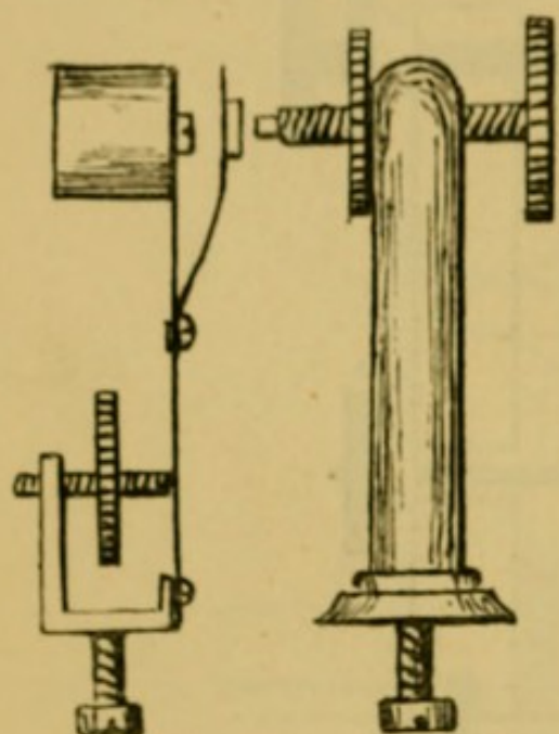
FIG. 14.—DOUBLE SPRING CONTACT-BREAKER.
