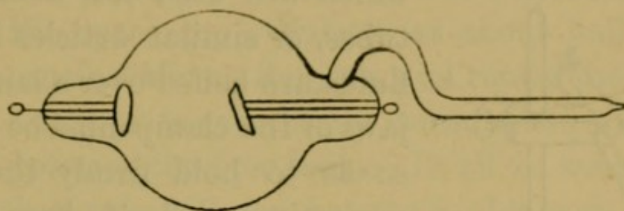
FIG. 27.—JACKSON FORM OF CROOKS' TUBE.
