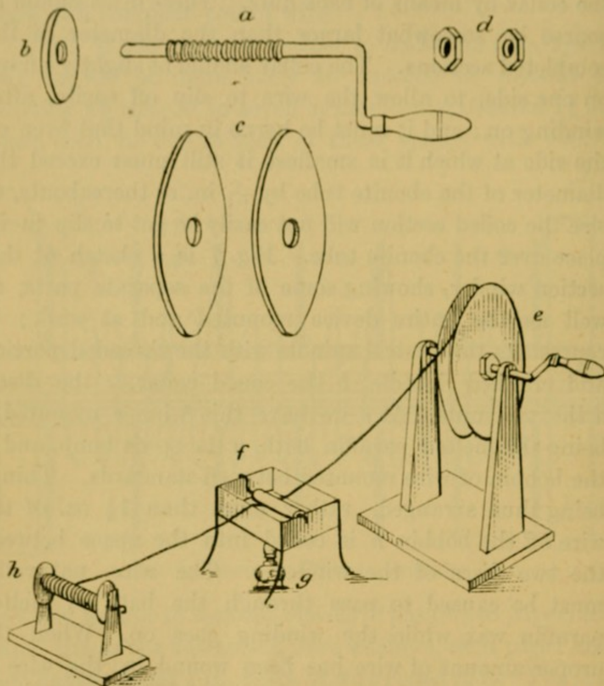
FIG. 7.—SECTION WINDER, SHOWING PARTS.
