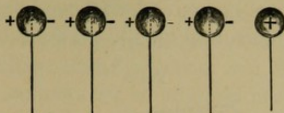
Electrical induction.
