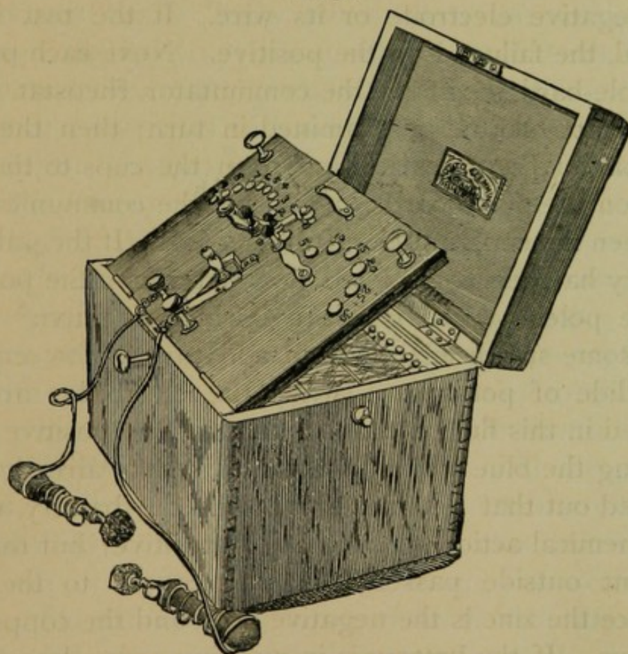
Portable Leclanché as made by Flemming.
