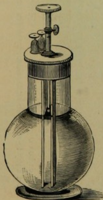
Grenet cell.
