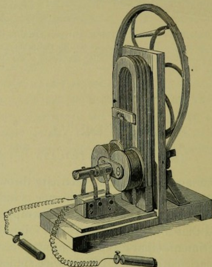
Magneto-electric battery. In this battery the magnets are placed vertically, and the coils are made to revolve rapidly by the large wheel.
