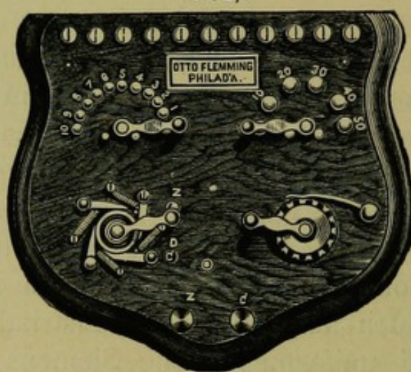
Flemming's key-board.
