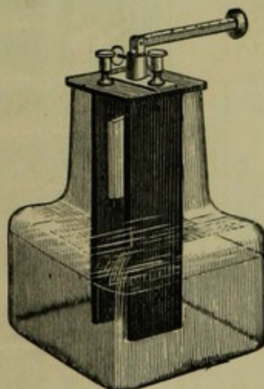
Another form of Grenet's cell.
