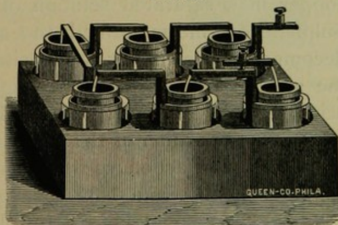
Grove's battery.
