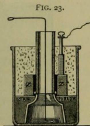
Siemens and Halske's modification of the Daniell element, as made for Remak.
