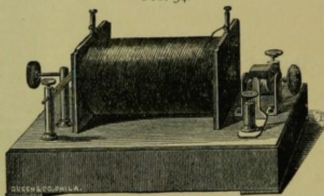
Ruhmkorff's coil.
