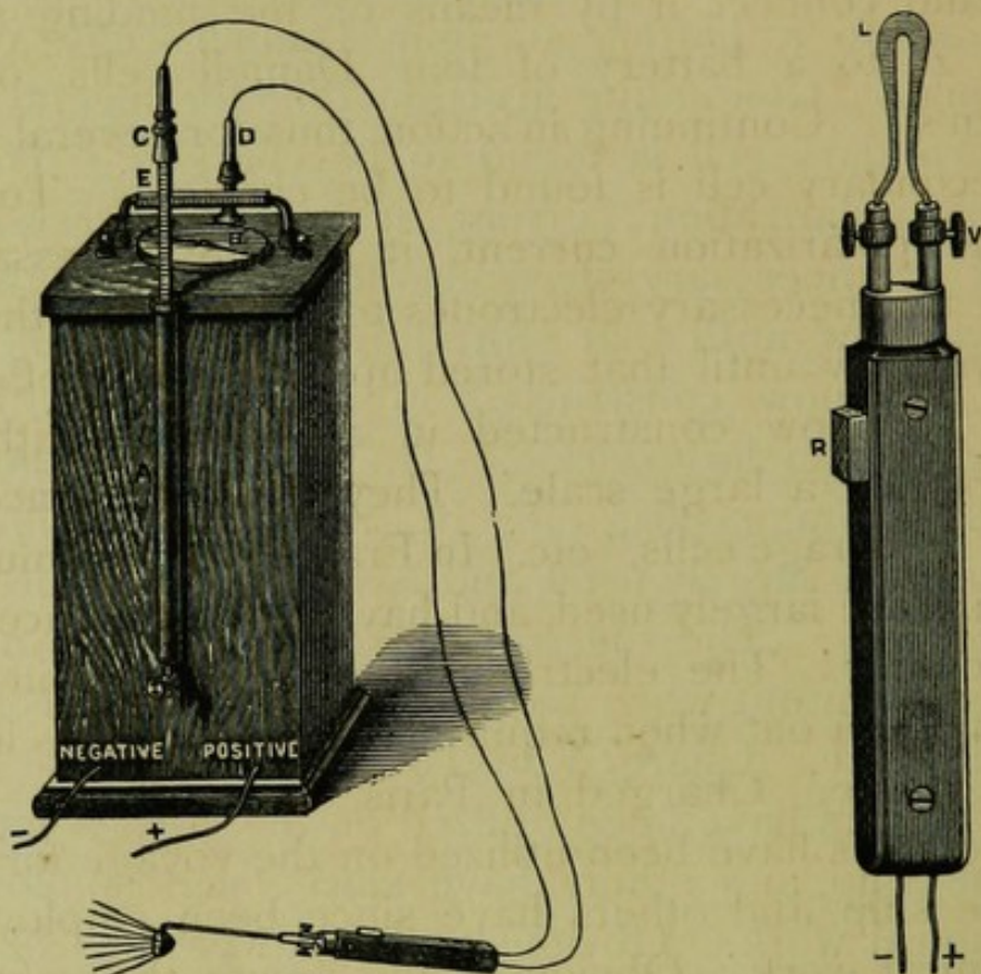
Trouvé's polyscope.
