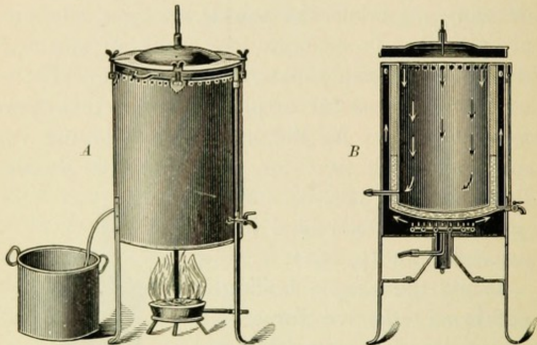
FIG. 27.—Lautenschläger's steam sterilizer for dressings ( A , exterior view, B , cross-section).
