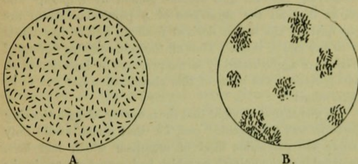
Fig. 3.—Diagrammatic representation of agglutination. A, Free bacilli ; B, Bacilli agglutinated.
