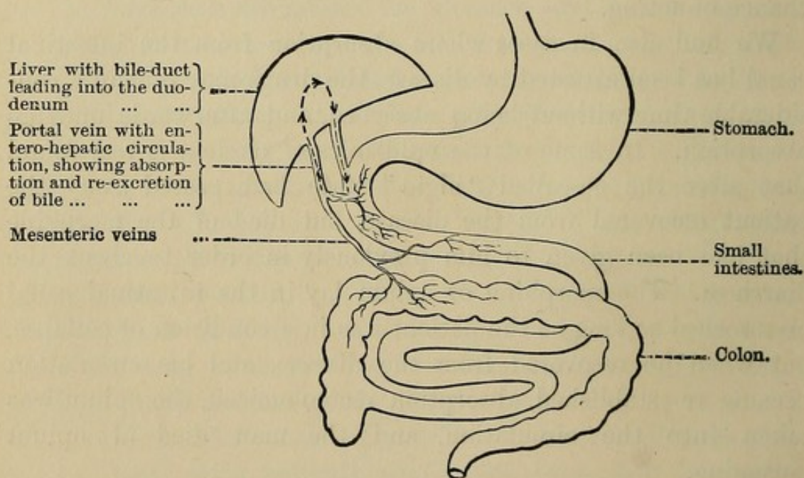
FIG. 3.—Entero-hepatic Circulation.
