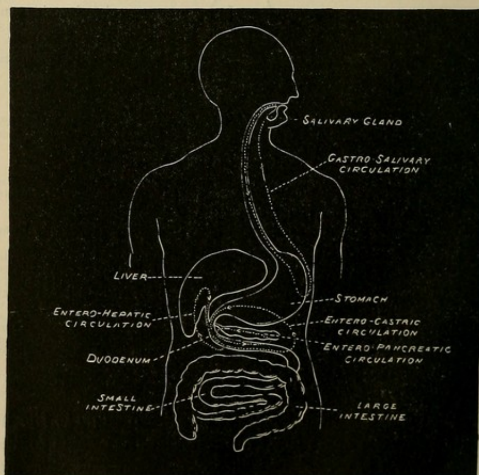
FIG. 5.—Gastro-salivary—Entero-gastric—Entero-hepatic—Entero-pancreatic circulation.
