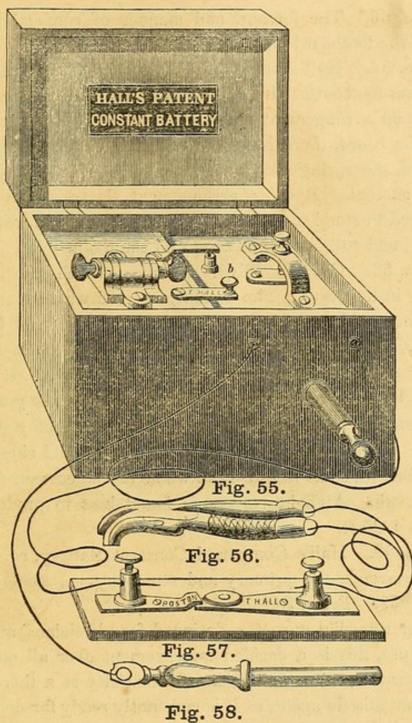
No. 55. Hall's Patent Constant Battery for Extracting Teeth without pain. Represents the instrument complete in box. Price, $12.00.
