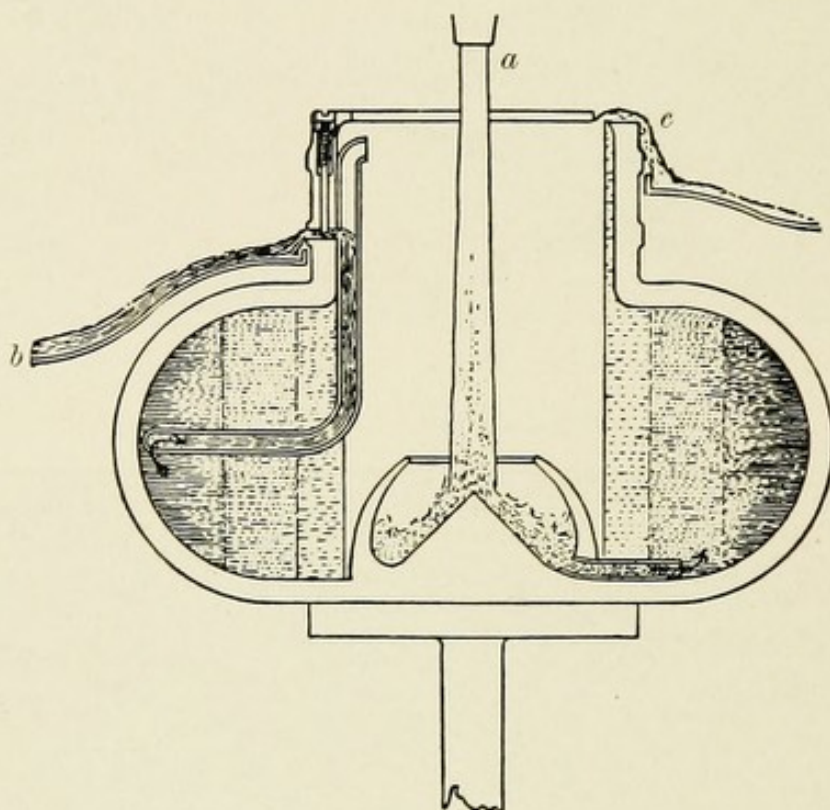
FIG. 10.—Centrifugal Cream Separator. (Wing.) a , Inflowing milk ; b , outflowing skimmed milk ; c , outflowing cream.
