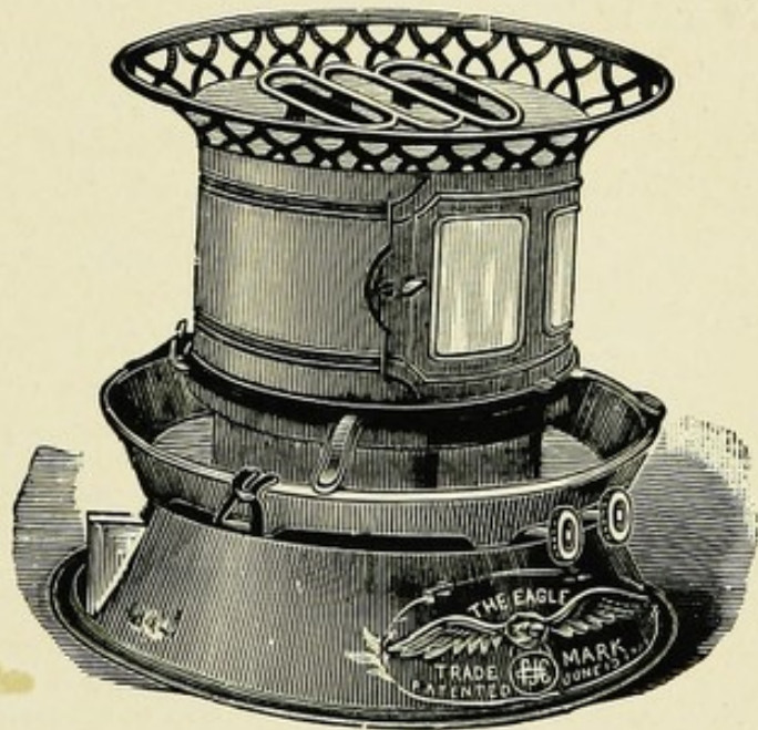
FIG. 69. Oil Stove for Nursery.
