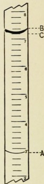
FIG. 32.—Fat in Neck of Test Bottle. Reading should be made between A and B not between A and C. (Wing.)
