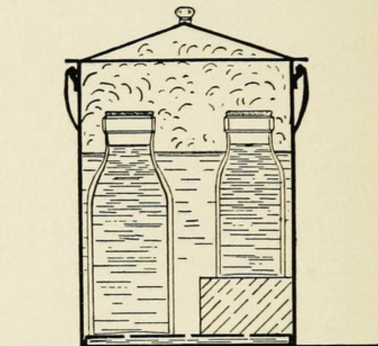
FIG. 63.—Pasteurizer for Bottled Milk. (Russell.)
