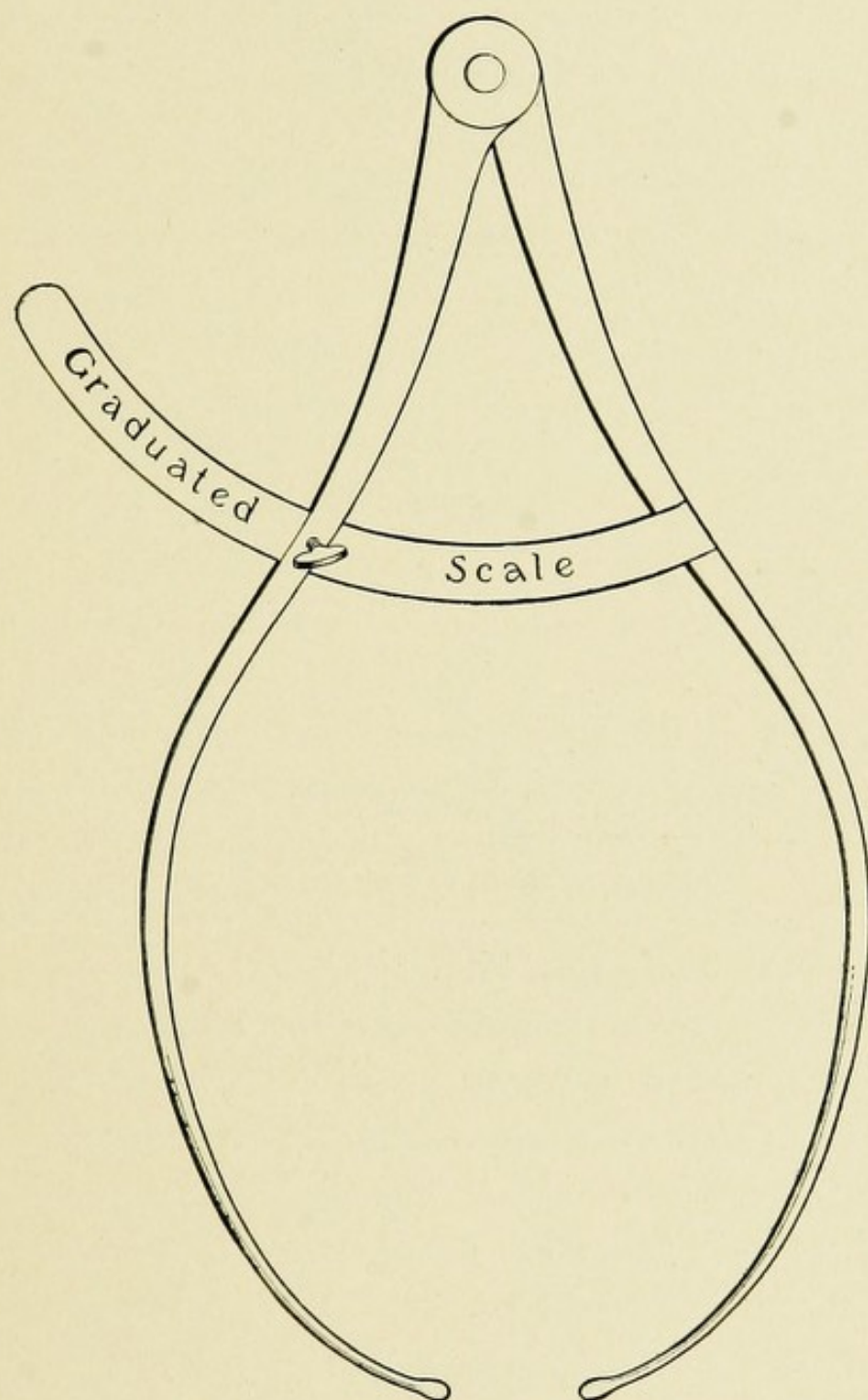
FIG. 89.—French Calipers.
