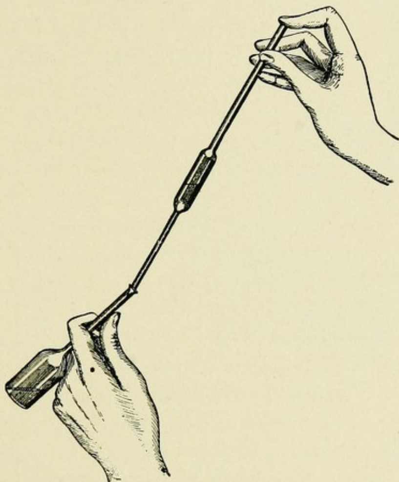
FIG. 30.—Right Way of Emptying Pipette. (Farrington and Woll.)
