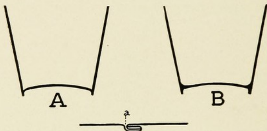
FIG. 20.—A, Improper joints in dairy utensils. B, Proper joints closed with solder. (After Russell.)
