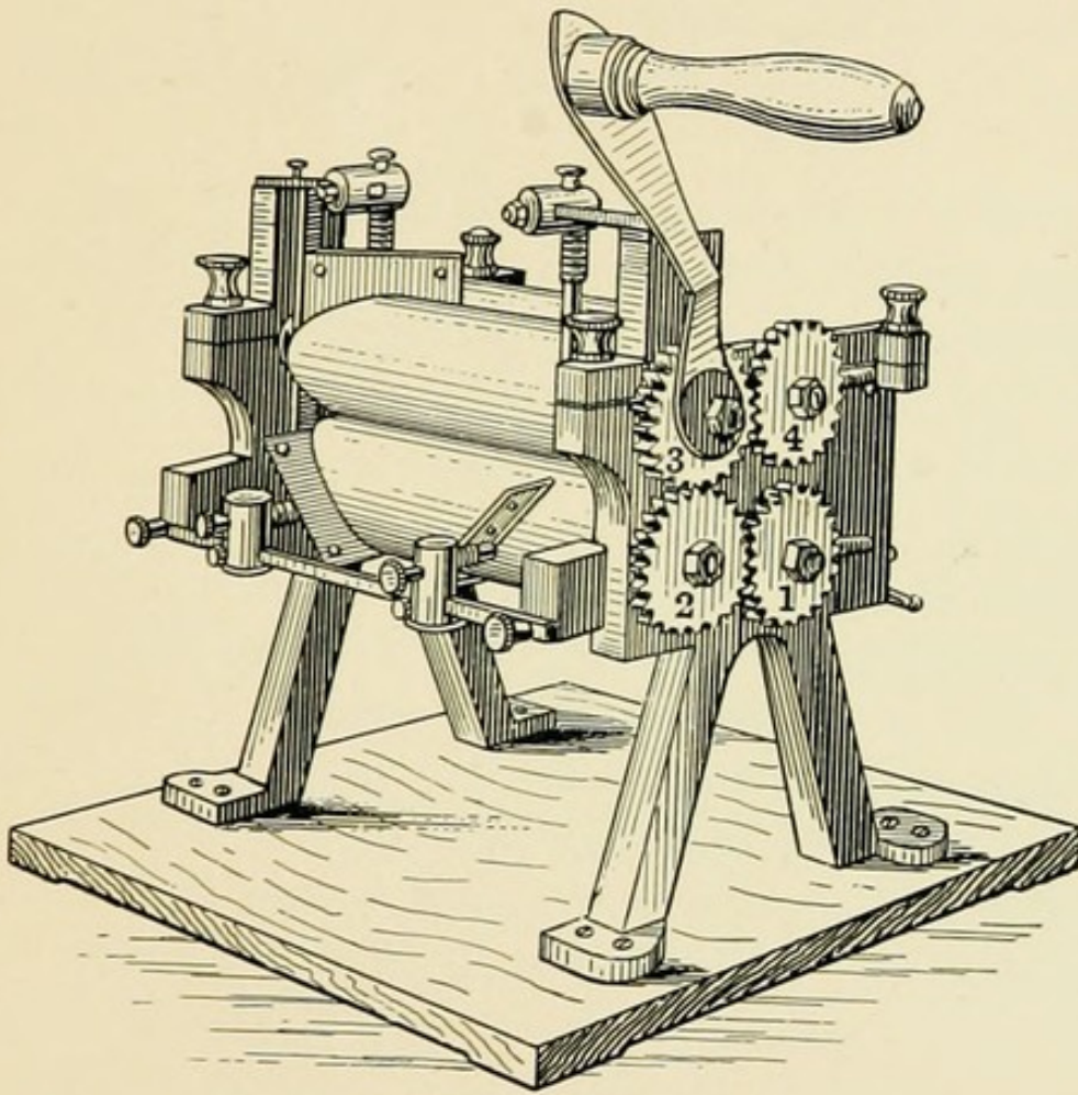
Lymph-mixing machine of Dr. Döring, Berlin.
