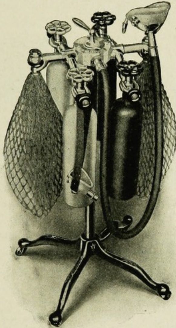
THE CLARK NEW MODEL OXYGEN AND NITROUS OXID GAS APPARATUS.
