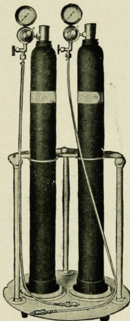
NO. 1 PORTABLE STAND, WITH STYLE F CYLINDERS.
