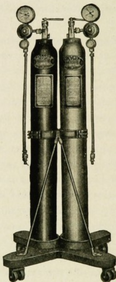
NO. 2 LENNOX STAND.
