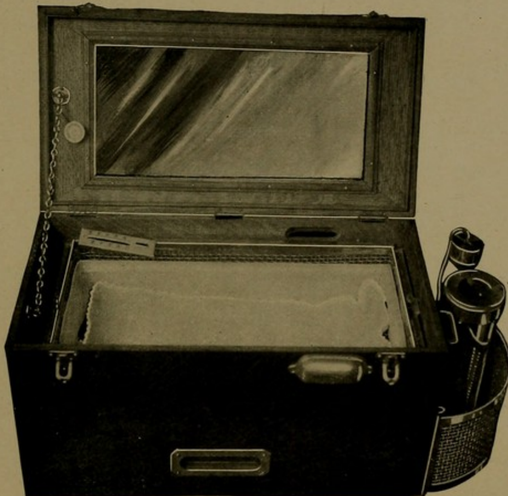
FIG. 139.—Incubator ambulance open, showing electric light, thermometer, infant's basket with eiderdown flannel mattress and coverlet.
