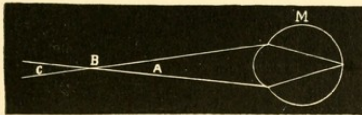
Rays coming from a myopic eyeball.
