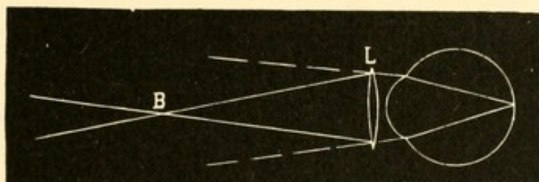
Rays emerging from a hypermetropic eye.
