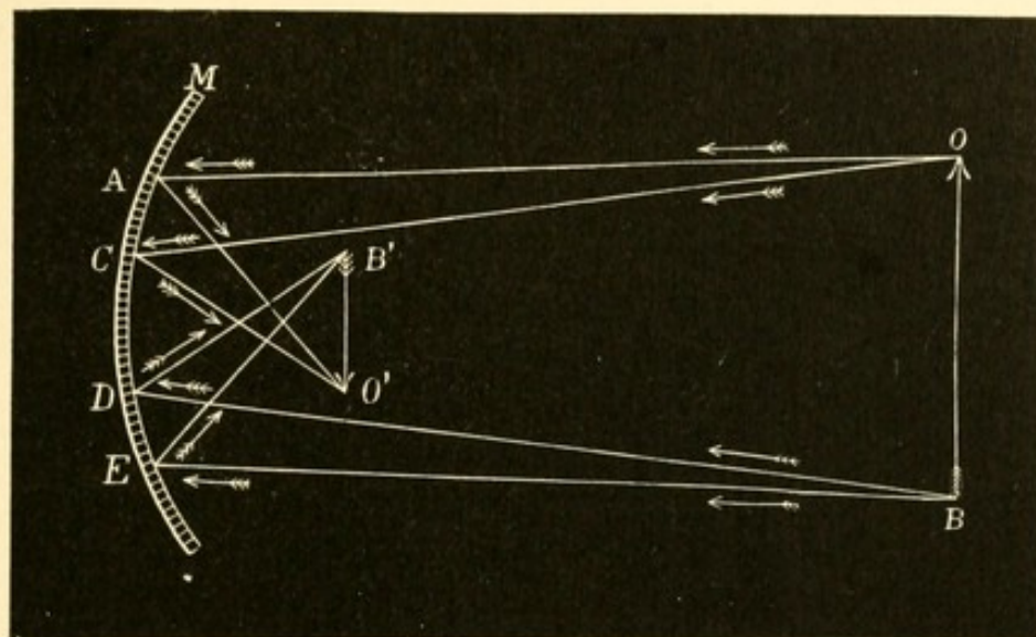
Reflection from a concave mirror.
