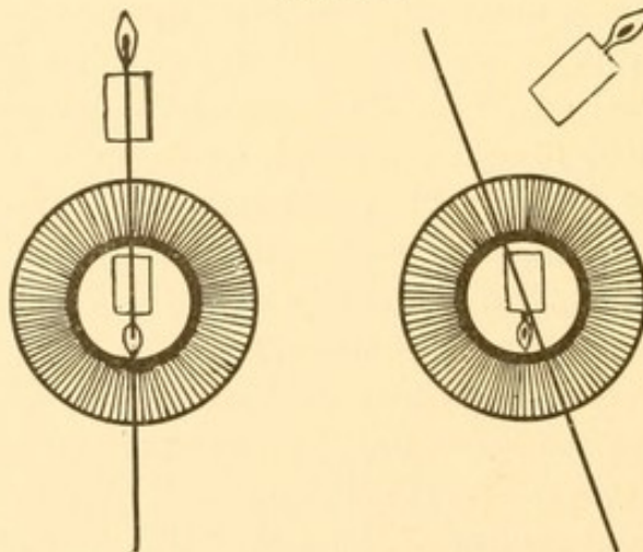
Vertical meridian of left eye converging by its upper extremity.
