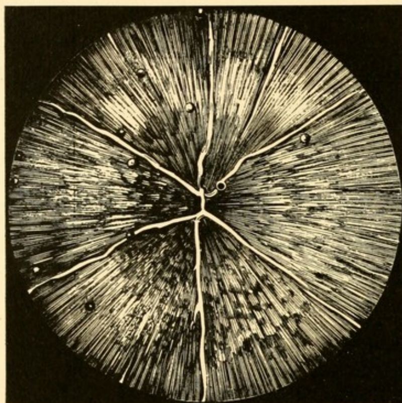
Spectrum of lens showing sectors. (Donders.)
