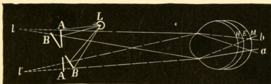
Retinoscopy with the plane mirror.
