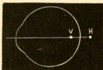
Foci of the principal meridians in mixed astigmatism.
