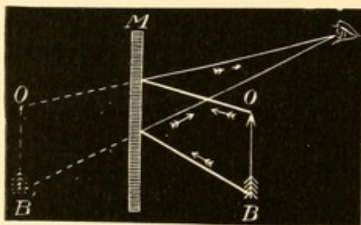
Reflection from a plane mirror.
