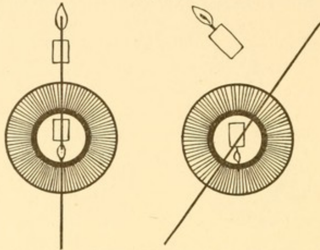
Vertical meridian of left eye diverging by its upper extremity.
