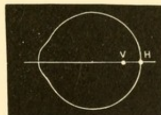
Foci of the principal meridians in simple myopic astigmatism.
