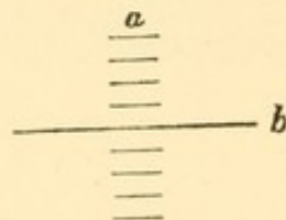
Horizontal lines focused by emmetropic vertical meridian.
