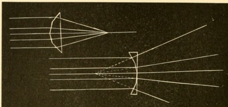
Lenses as prisms.
