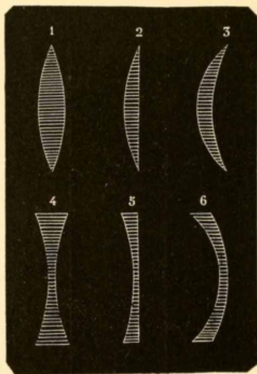
1. Biconvex lens. 2. Plano-convex lens. 3. Concavo-convex lens, convergent meniscus. 4. Biconcave lens. 5. Plano-concave lens. 6. Convexo-concave lens, divergent meniscus.
