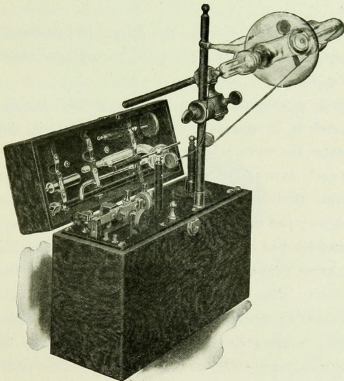
Fig. 40. Portable Coil.
