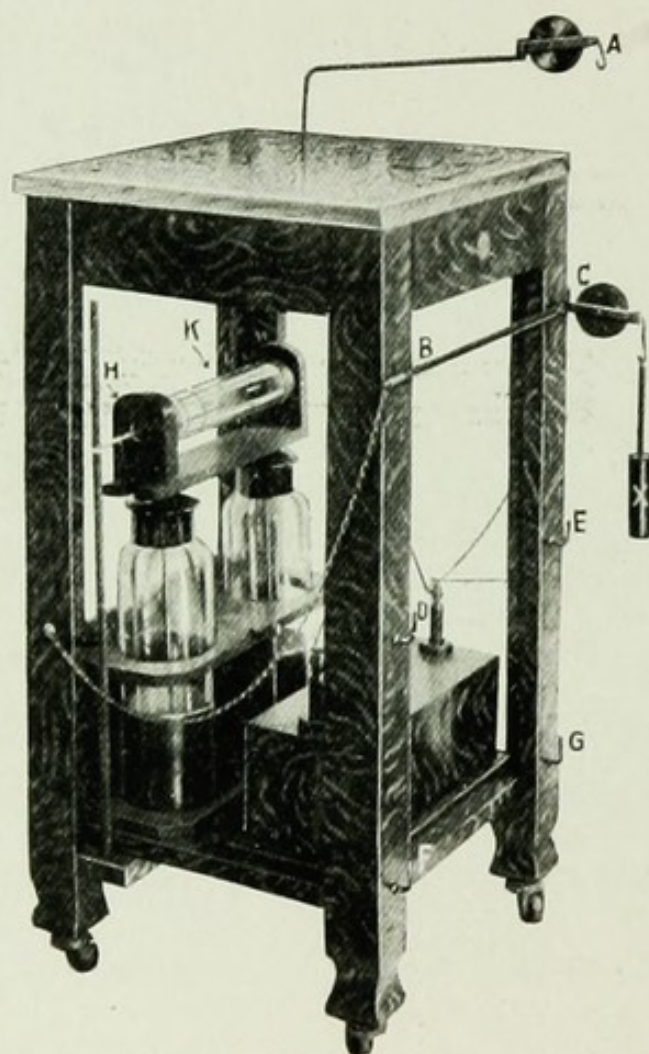
Fig. 6. Resonator.
