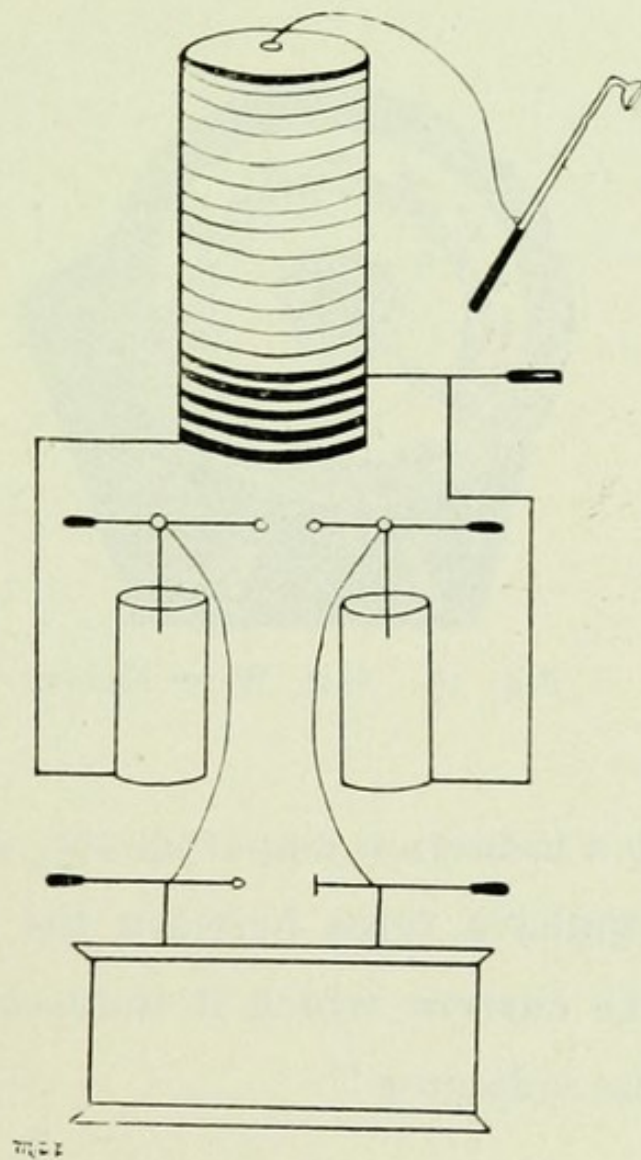
Fig. 15. Diagram of Oudin Resonator.
