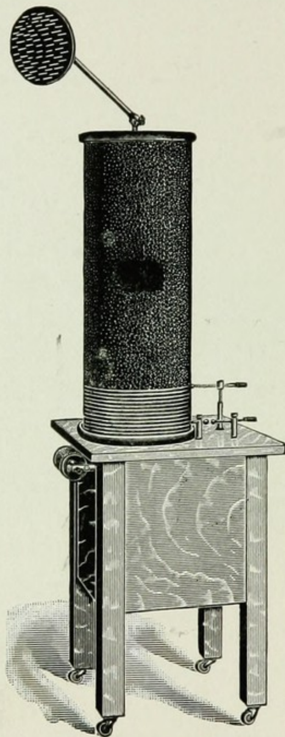
Fig. 61. D'Arsonval-Oudin Resonator.
