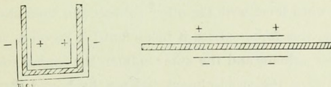
Fig. 8. Section of Jar. Fig. 9. Section of Plate Condenser
