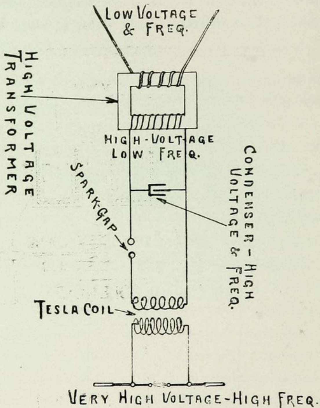
Fig. 14. Diagram of Tesla Type.
