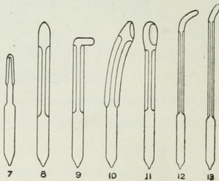
Fig. 21. Insulated Tubes.
