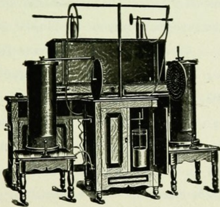
Fig. 30. Double Resonators with Diaphragms.
