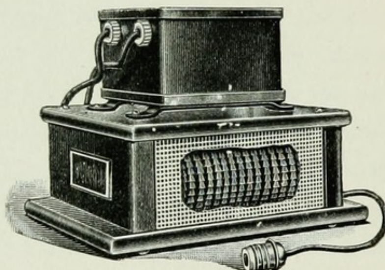
Fig. 58. Ozone generator for ozonizing the air of a room.
