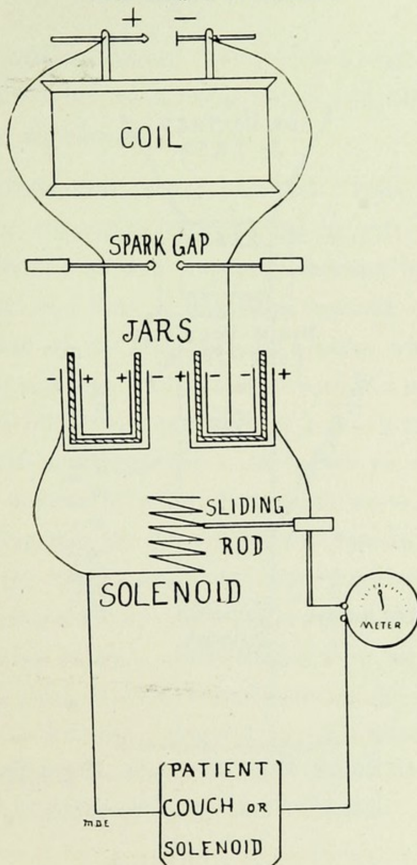
Fig. 13. Diagram of D'Arsonval Type.
