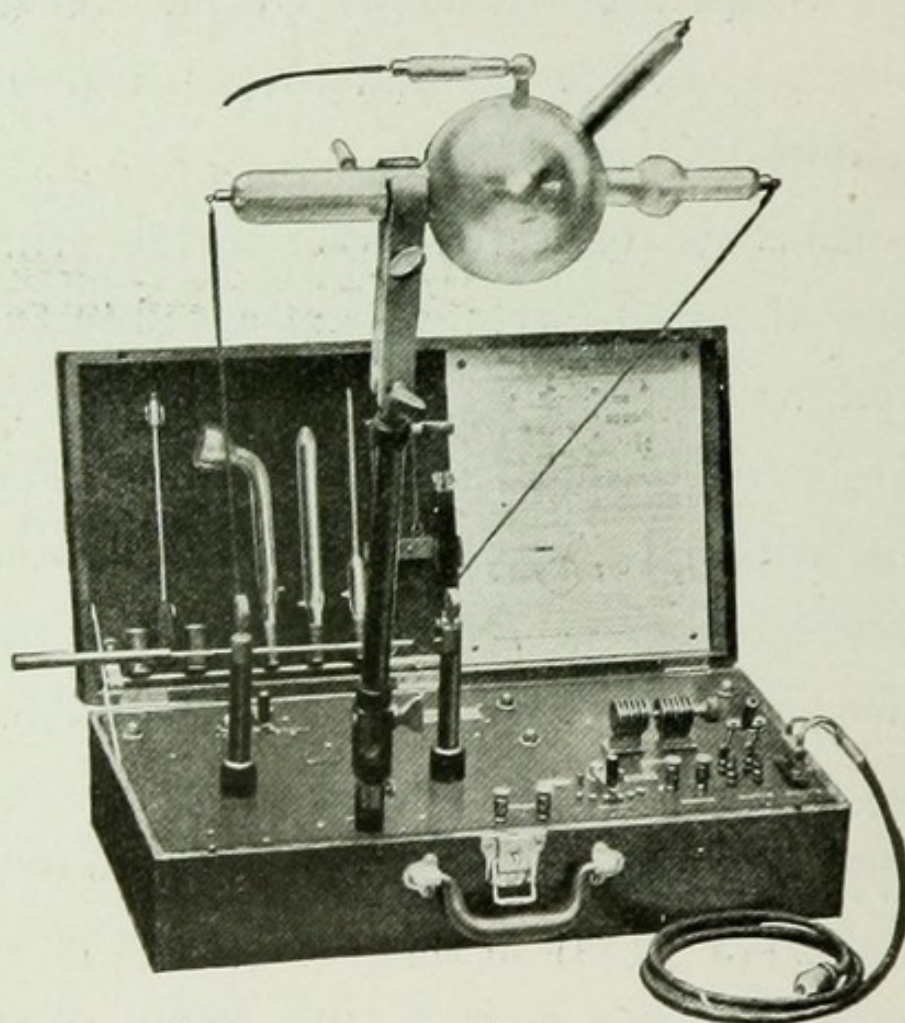
Fig. 39. Portable Coil.
