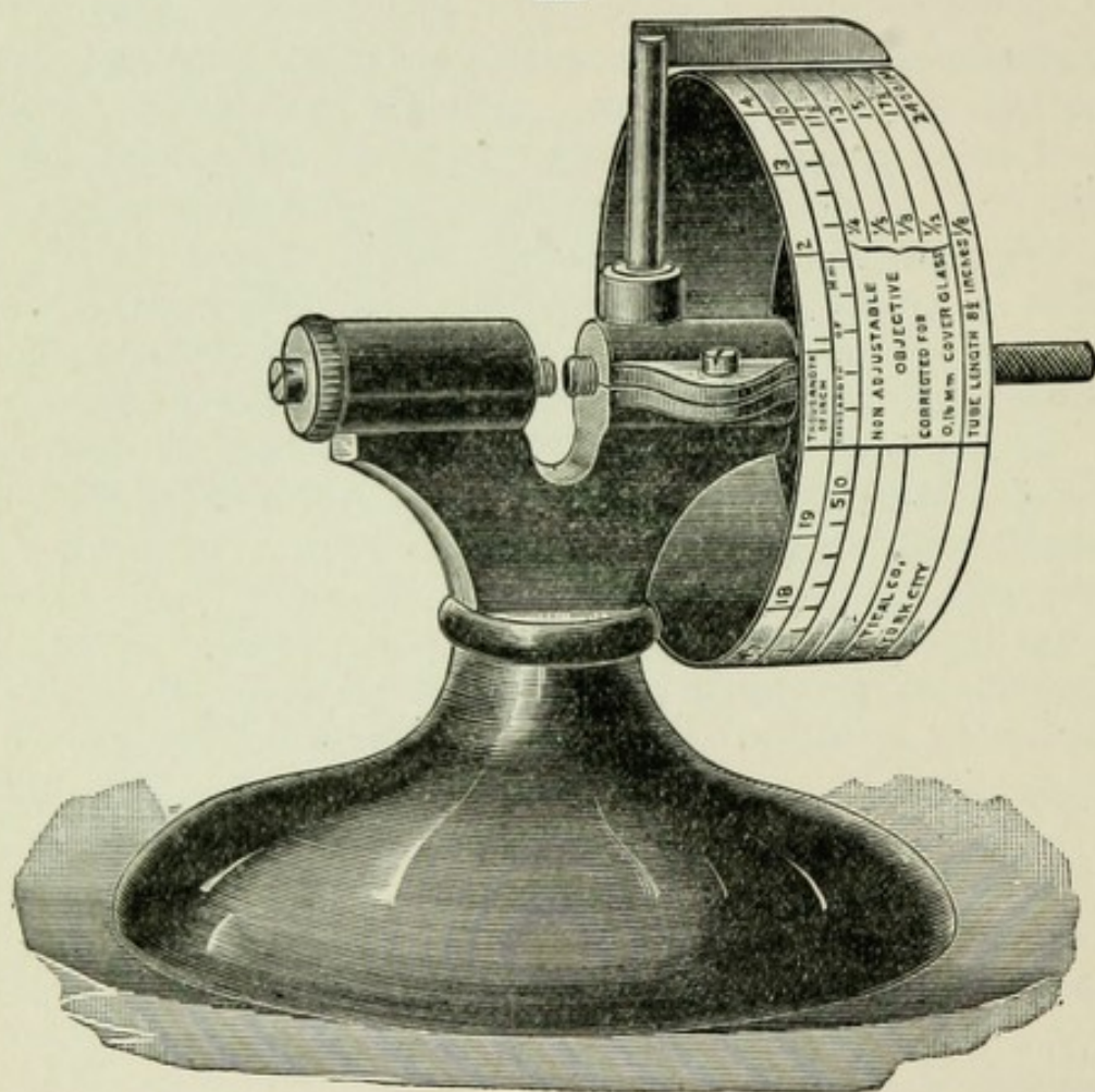
Fig. 38. Cover-Glass Measurer (Edward Bausch).
