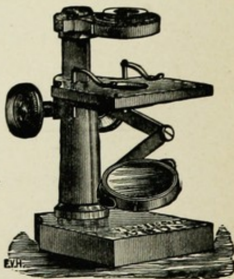
FIG. 8a. — Simple Microscope with Special Mechanical Mounting to Hold and Focus the Magnifier and to Support and Light the Object.
