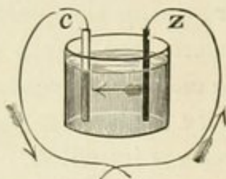
FIG. 1.—Simple Battery.
