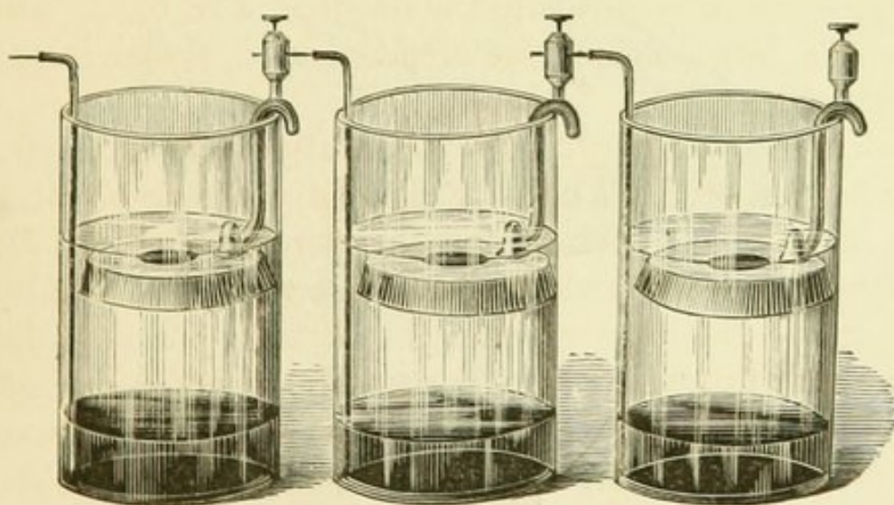
FIG. 6.—Hammond's Permanent Battery.
