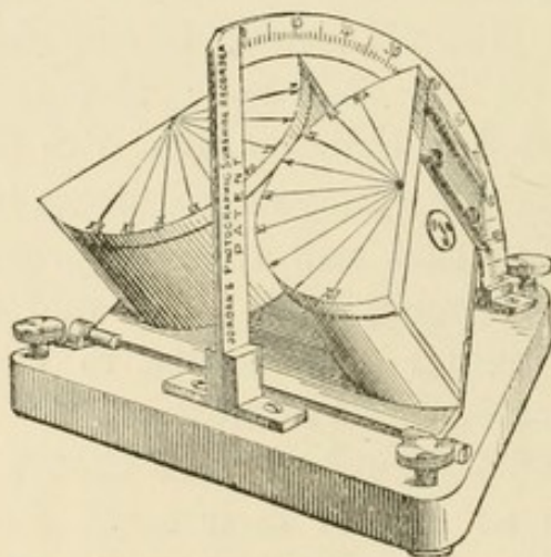
THE JORDAN PHOTOGRAPHIC SUNSHINE RECORDER.
